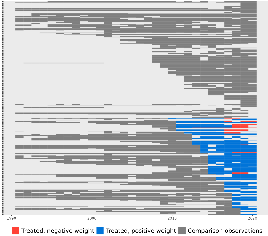
Figure B2: TWFE negative weights in classic TWFE regression reported in Column (2) of Table 2
