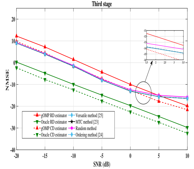
FIGURE 5: NMSE performance results of mmWave channel estimation at the third stage vs. SNR of the proposed joint design method, the method random design [26] via gOMP, Oracle algorithms by using G = 100 compared with other methods based on codebook schemes by using G = 160 as codebook based minimal total coherence (MTC) scheme [23], codebook based ordering scheme [24], codebook based Versatile scheme [25], codebook based random scheme.
