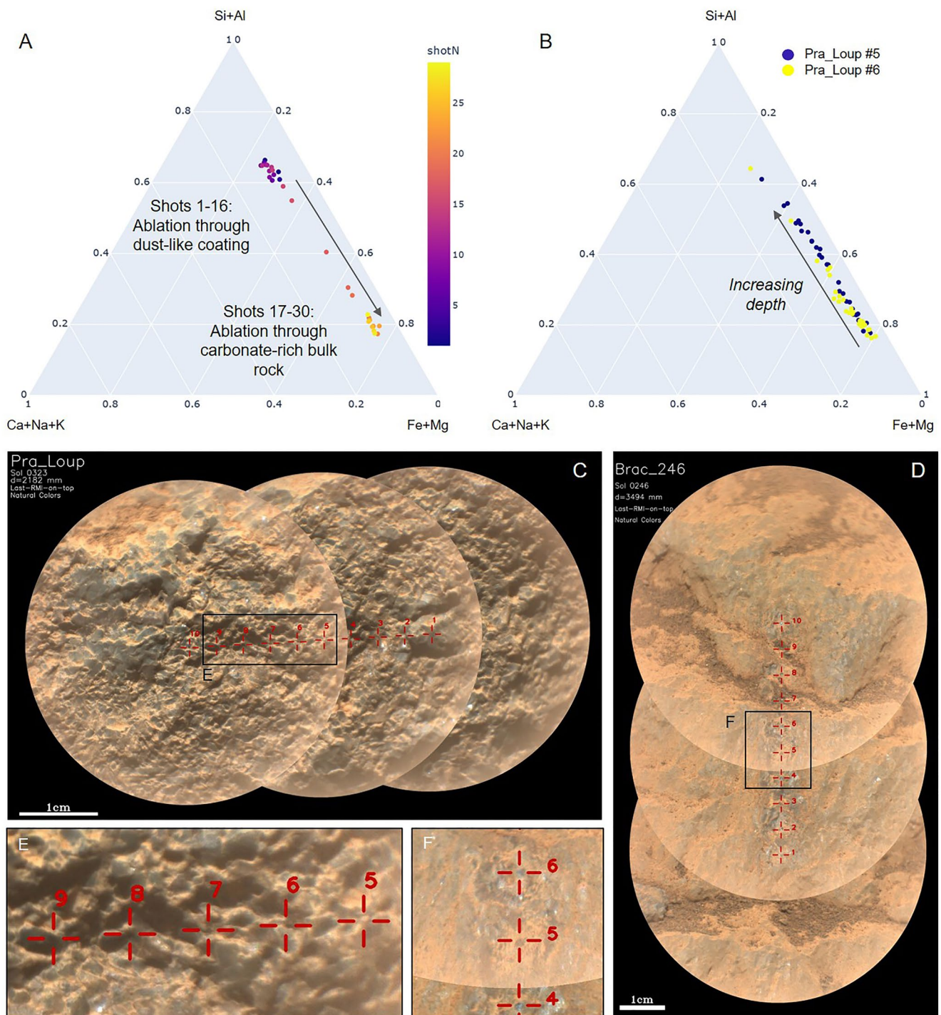
Figure 6. (a–b) Compositional depth trends (molar composition); the arrows indicate increasing depth (a) Brac_246 #5 shot-to-shot composition data, showing two different mineral phases probed in the first ~15 and last ~15 shots; (b) Pra_Loup #5 and #6, showing similar mixing trends; the Si content increases with depth. (c–f) RMI images of the Pra_Loup and Brac_246 targets; close-ups of points of interest in E and F; point #9 of Pra_Loup sampled an olivine grain.
