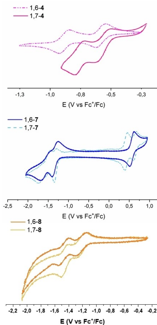
Figure 6. Cyclic voltammetry of dyes 4 , 7 (in \text{CH}_2\text{Cl}_2 ), and 8 (in \text{CHCl}_3 ), scanned toward negative potentials, with n\text{-Bu}_4\text{NPF}_6 (0.1 M) as electrolyte.
