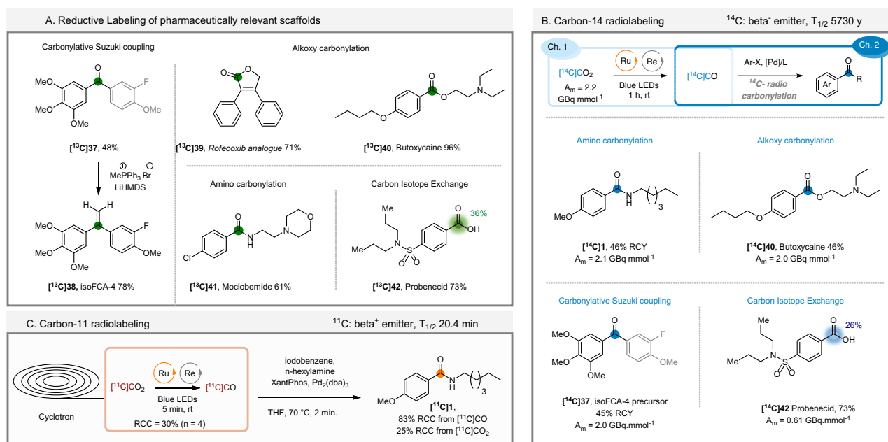
Fig. 5 | Application of the photocatalytic \text{CO}_2 -to- \text{CO} conversion to ^{13}\text{C} , ^{14}\text{C} and ^{11}\text{C} carbonylation. A Labeling of pharmaceutically relevant scaffolds. B Carbon-14 radiolabeling. C Carbon-11 radiolabeling. See Supplementary pages 86–109, for
