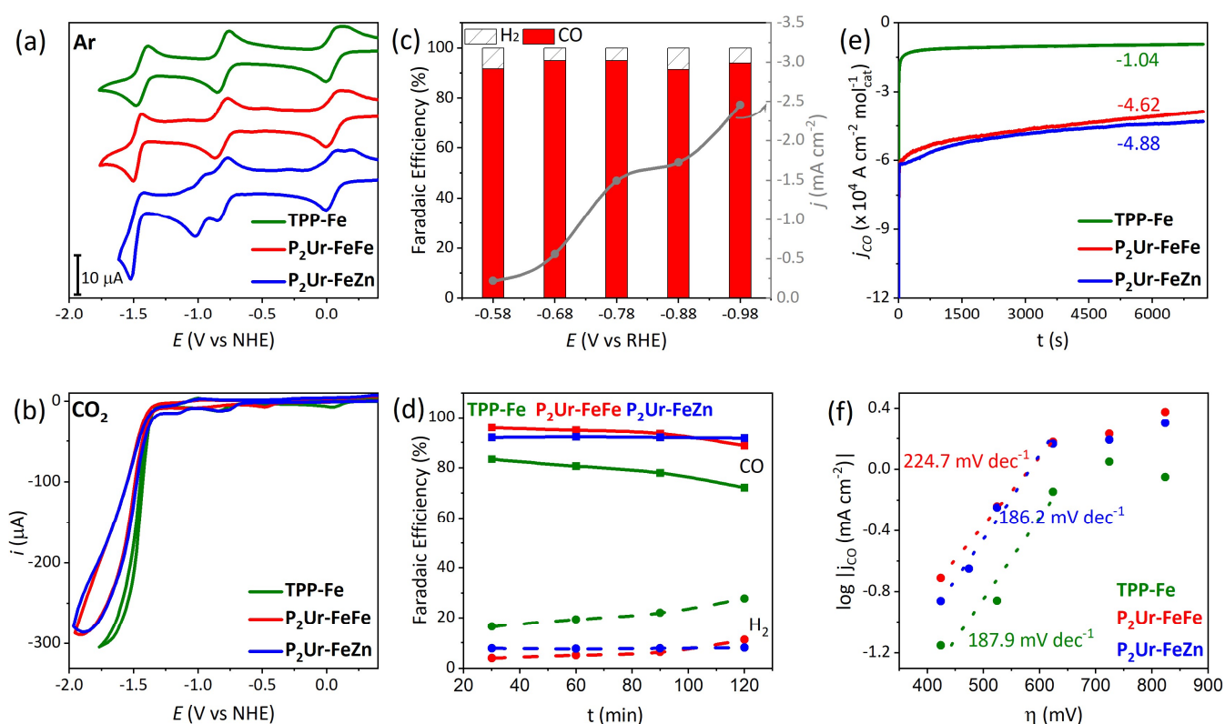
Figure 2. Cyclic voltammograms (CVs) of the complexes TPP-Fe (green), P 2 Ur-FeFe (red) and P 2 Ur-FeZn (blue) (a) under Ar-saturated homogeneous DMF solution with 0.1 M [Bu 4 N]PF 6 (b) under CO 2 saturation (bottom) with 5.5 M H 2 O. (c) Potential-dependent selectivity and current density of P 2 Ur-FeFe -modified CNT/CP electrode in CO 2 -saturated 0.1 M aqueous NaHCO 3 solution. Comparison of (d) Faradaic efficiency, (e) CO partial current density and (f) Tafel plot of heterogenized TPP-Fe (green), P 2 Ur-FeFe (red) and P 2 Ur-FeZn (blue).
