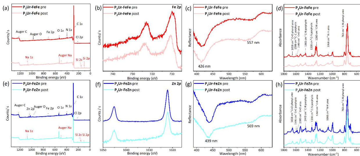
Figure 3. (a, e) XPS survey spectra, (b, f) metal (Fe 2p or Zn 2p) high resolution spectra, (c, g) UV-Vis spectra (d, h) ATR-FTIR spectra analyses of the P 2 Ur-FeFe and P 2 Ur-FeZn modified CNT/CP electrodes before (red: P 2 Ur-FeFe , blue: P 2 Ur-FeZn ) and after heterogeneous CO 2 electrolysis (pink: P 2 Ur-FeFe , cyan: P 2 Ur-FeZn )
