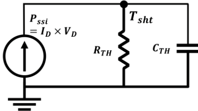
Fig. 5. RC filter-like electrical equivalent circuit for the implementation of self-heating effects.
