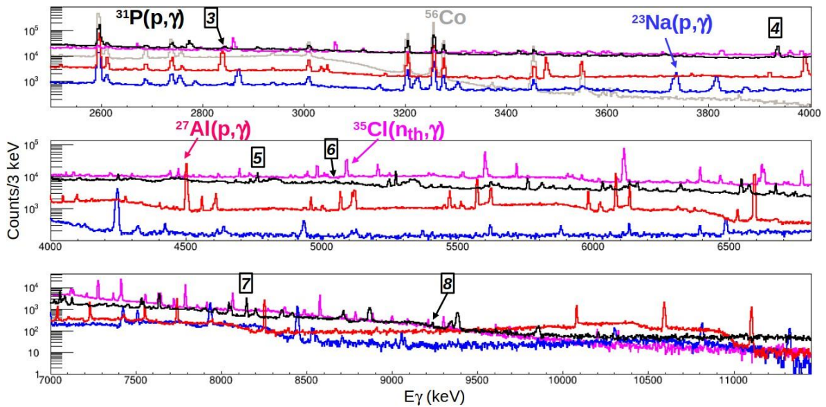
Figure 3. (Color online) Selection of \gamma -ray spectra obtained with the \vartheta=-90 HPGe detector and the digital DAQ. Labels 3 to 8 refer to the \gamma -ray lines from the ^{32}\text{S}^{IAS} state. The coloured spectra were obtained in (p,\gamma) and (n_{th},\gamma) calibration runs.
