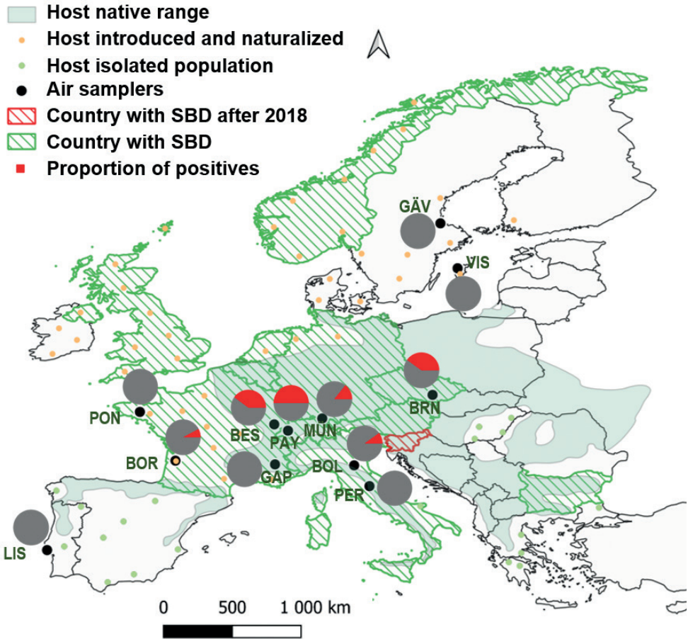
Figure 6. Proportion of aerobiological samples that tested positive from May to September of 2018 ( n = 10 , except for Gap where n = 5 ) in the different European samplers following the natural distribution of the host Acer pseudoplatanus .
