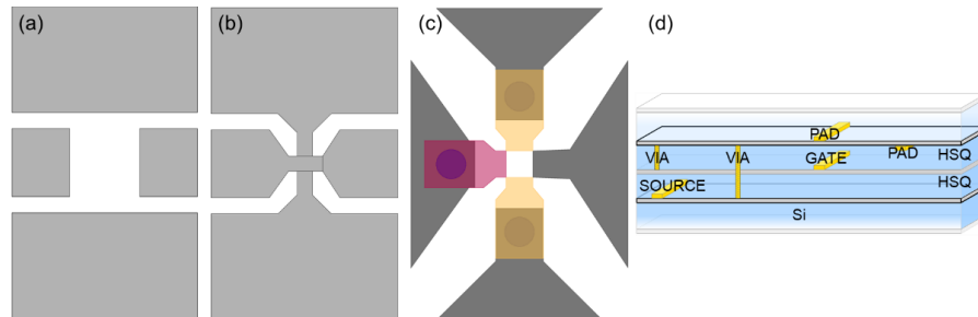
Figure 3: Virtual structures for the EM simulation, a) OPEN_PAD, b) SHORT_PAD, c) OPEN_DUT and (d) the substrate definition on ADS for EM simulation.
