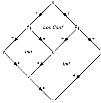
Figure 2: Huet's original diagram for the proof
