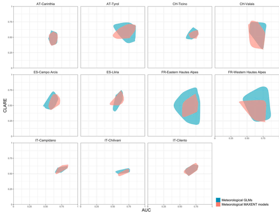
Fig. 5. Comparison of the meteorological GLM and Maxent models for all regions. To enhance the readability, in the plots multi-variable model performances are represented by lines encompassing the entire range of models (models with 2 or more explanatory variables). Larger bubbles indicate that the performance of the multi-variable models is distributed over a larger area, while smaller bubbles indicate a narrower distribution.
