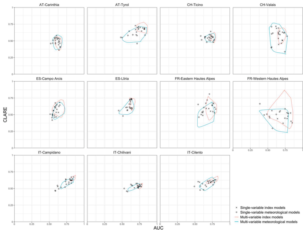
Fig. 3. CLARE vs. AUC performances of the Maxent models for all regions. To enhance the readability, in the plots multi-variable model performances are represented by lines encompassing the entire range of models (models with 2 or more explanatory variables). The symbols represent all single variable models.
