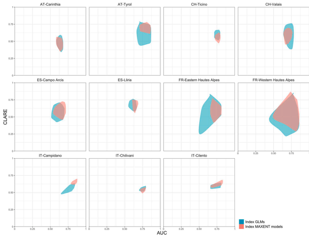
Fig. 4. Comparison of the fire weather GLM and Maxent models for all regions. To enhance the readability, in the plots multi-variable model performances are represented by lines encompassing the entire range of models including single and multi-variable models. Larger bubbles indicate that the performance of the multi-variable models is distributed over a larger area, while smaller bubbles indicate a narrower distribution.
