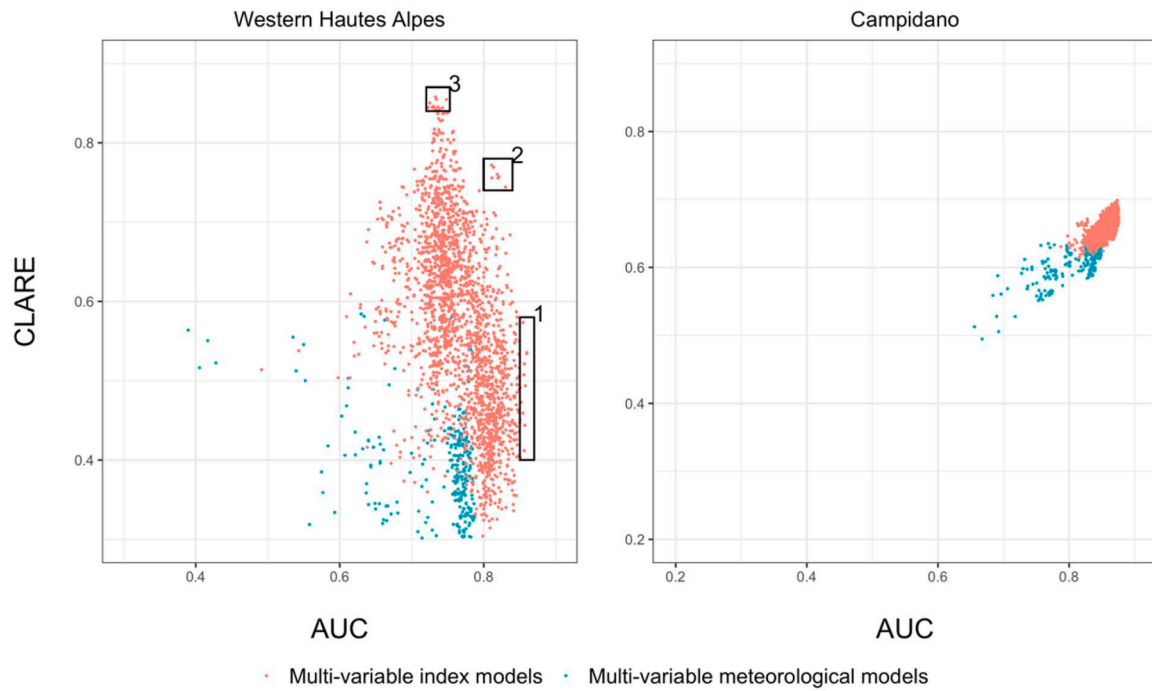
Fig. 2. CLARE vs. AUC performances of all index and meteorological models for Western Hautes Alpes and Campidano. Numbered boxes highlight the highest performance in AUC (box 1), CLARE (box 3), and both metrics (box 2).
