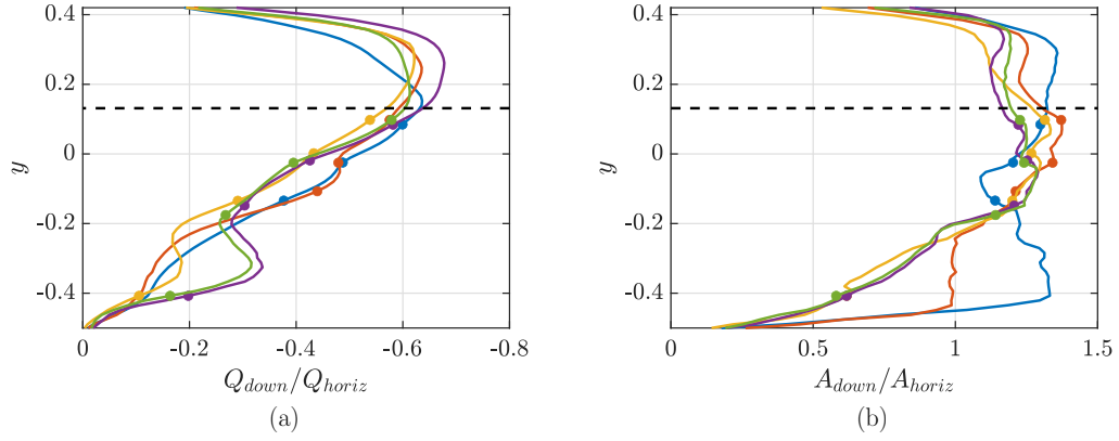
FIG. 8. (a) Vertical profiles of the ratio between the downward and horizontal flow rates Q_{down}/Q_{horiz} (with Q_{horiz} = \langle \bar{u}_\theta \rangle_{r,\theta,y} HL ). The profiles, obtained using Eq. (9), are shown for Gr_{ac} = 1.78 \times 10^4 (blue), Gr_{ac} = 3.64 \times 10^4 (orange), Gr_{ac} = 7.50 \times 10^4 (yellow), Gr_{ac} = 11.28 \times 10^4 (purple) and Gr_{ac} = 15.12 \times 10^4 (green). Note that the x -axis is reversed and that Q_{down} is counted negatively for downward motion. (b) Dimensionless cross-sectional area of downward-moving fluid A_{down} . The black dashed line locates the height at which the acoustic beam enters the cavity. The dots indicate the vertical positions of impingements of jets 1, 2, 3 and 5 in descending values of y , respectively.
