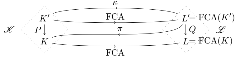
Figure 11: Relations between P and Q through the alternation of FCA and \pi (from [2021]).
