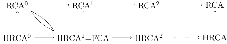
Figure 2: Relation between different restrictions of RCA (arrows mean: “can be rewritten into”).
