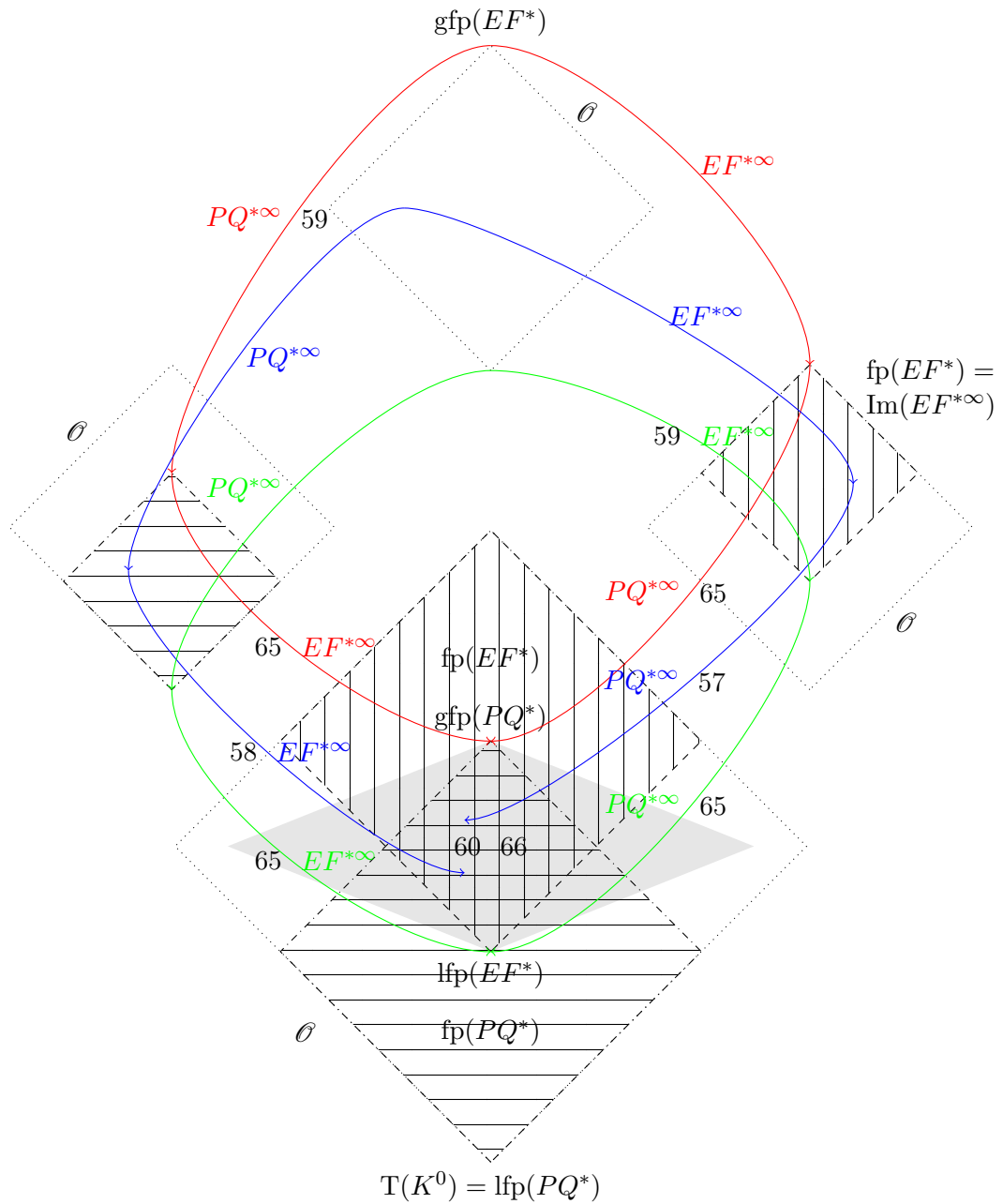
Figure 16: Illustration of Properties 57, 58, 59, 60, 61, 65 and 66. The figure displays four times \emptyset and the images of \text{gfp}(EF^*) (red), a random family of context-lattice pairs (blue) and \text{lfp}(PQ^*) = T(K^0) (green) through PQ^{*\infty} (left) and EF^{*\infty} (right). \text{fp}(EF^*) is drawn in vertical lines; \text{fp}(PQ^*) in horizontal lines and the grey area depicts the interval [\text{lfp}(EF^*) \text{gfp}(PQ^*)] .
