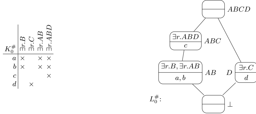
Figure 10: Non self-supported lattice L_0^\# .
