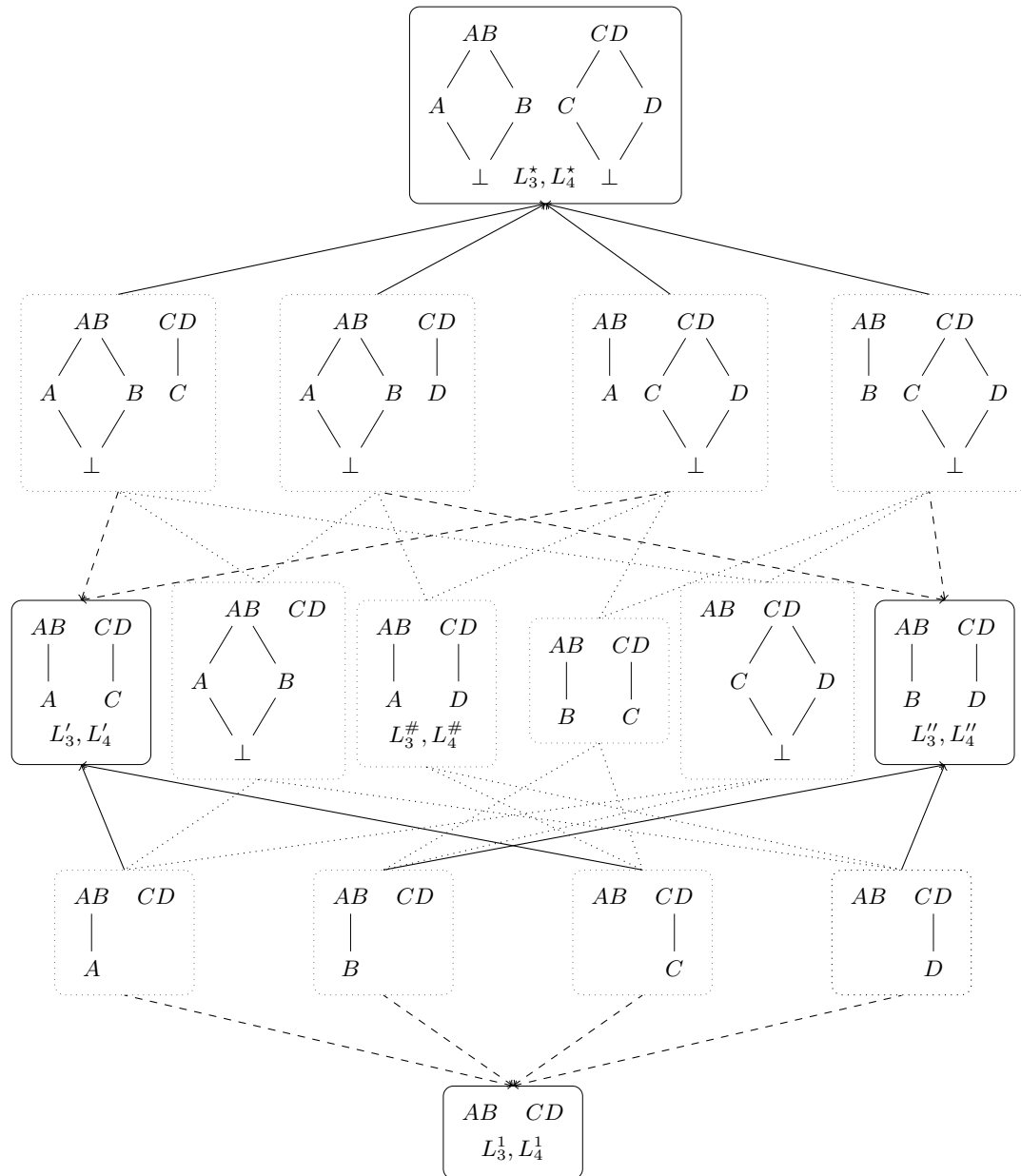
Figure 17: All the lattices belonging [\text{lfp}(EF^*) \text{ gfp}(PQ^*)] in the example of Section 3.3. Those in \text{fp}(EF^*) \cap \text{fp}(PQ^*) are within solid boxes. As usual, only direct edges are displayed. Solid arrows show direct most specific subsumers corresponding to EF^* and dashed arrows show direct more general subsumees corresponding to PQ^* .
