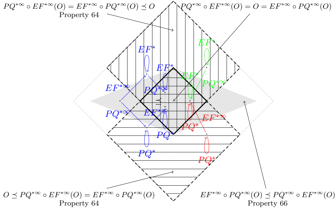
Figure 18: Illustration of the position of PQ^{*\infty} \circ EF^{*\infty} and EF^{*\infty} \circ PQ^{*\infty} depending on their original position (in dotted, \mathcal{O} , in dashed \text{fp}(EF^*) \cup \text{fp}(PQ^*) , in plain \text{fp}(EF^*) \cap \text{fp}(PQ^*) ). Colours corresponds to that of Figure 16: green starting from \text{fp}(EF^*) , red starting from \text{fp}(PQ^*) , blue starting outside of them.
