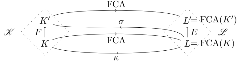
Figure 9: Relations between F and E through the alternation of FCA and \sigma_\Omega (from [2021]).
