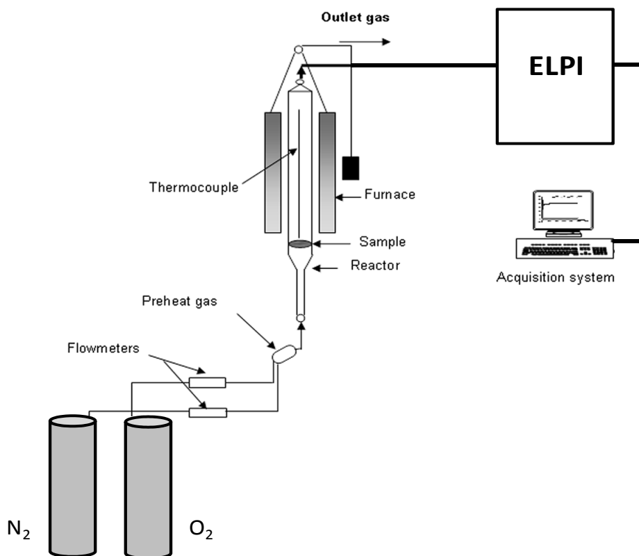
Fig. 2. Experimental device for combustion of date palm residues.
