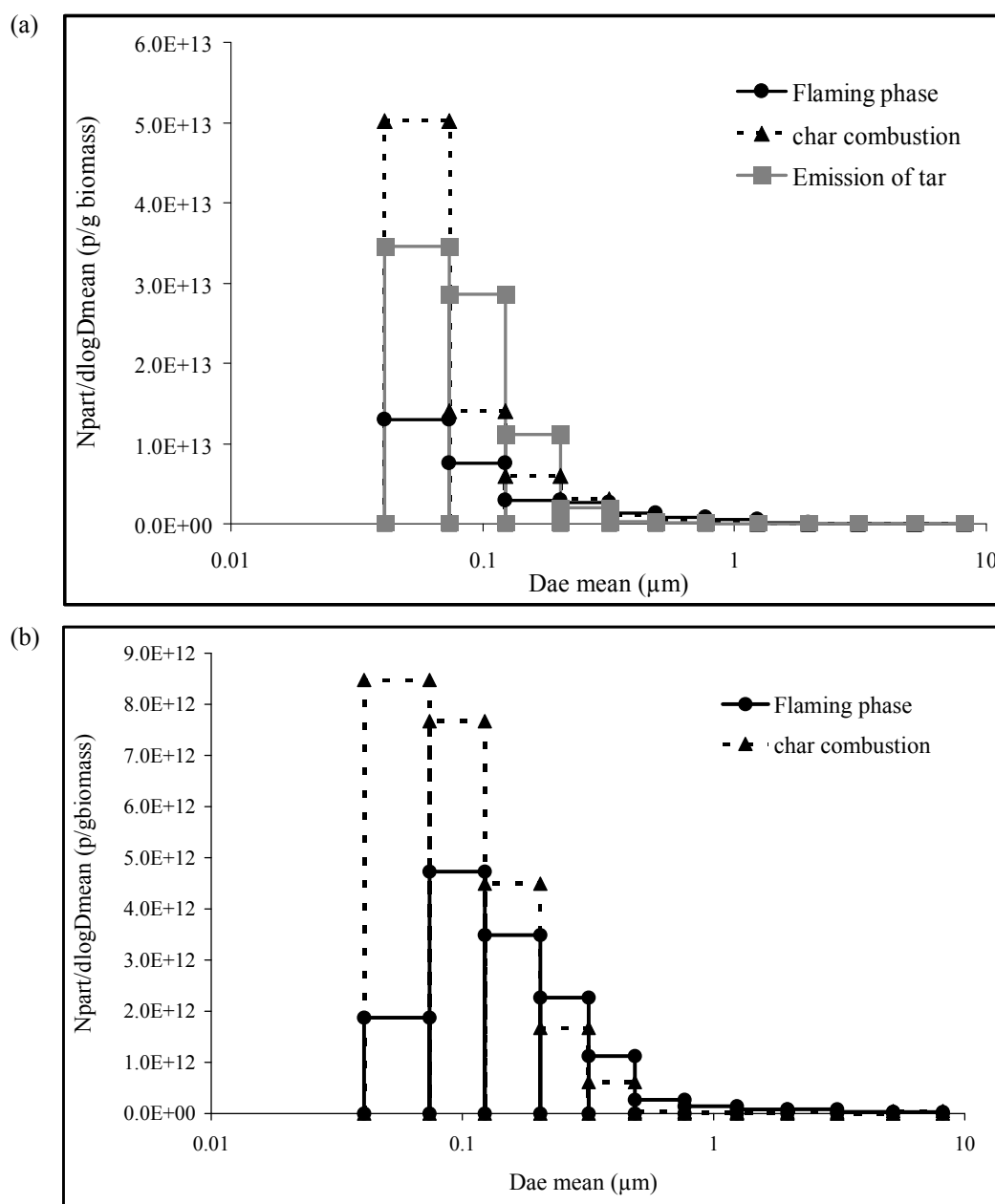
Fig. 7. Number size distributions of PM 10 for DS at (a) 500°C and (b) 800°C under an air flow rate of 50 NL/h.
