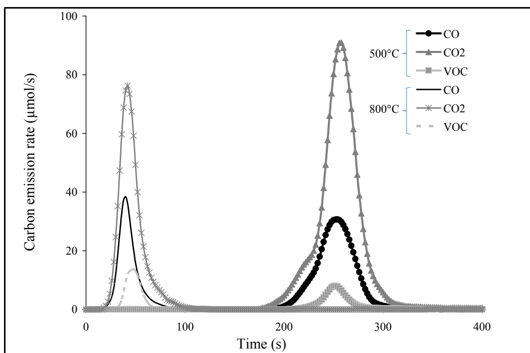
Fig. 4. Emission rates of carbon (CO, CO 2 and VOC) for DS at 500°C and 800°C.
