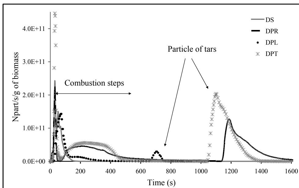
Fig. 5. Particle number emission rates as function of time during DPW combustions at 800°C.
