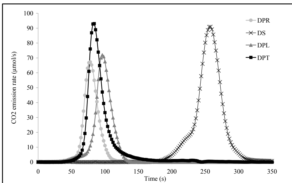
Fig. 3. Emission rates of CO 2 for DPW at 500°C.
