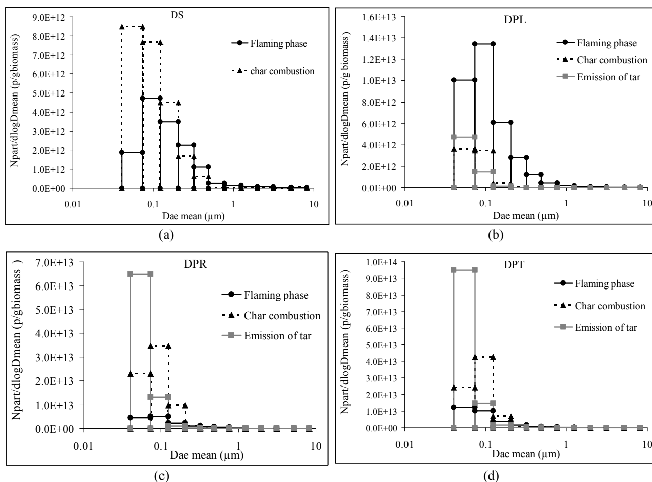
Fig. 8. Number size distributions of PM_{10} for (a) DS, (b) DPL, (c) DPR and (d) DPT during the different steps of the combustion at 800^{\circ}\text{C} under an air flow rate of 50 NL/h.
