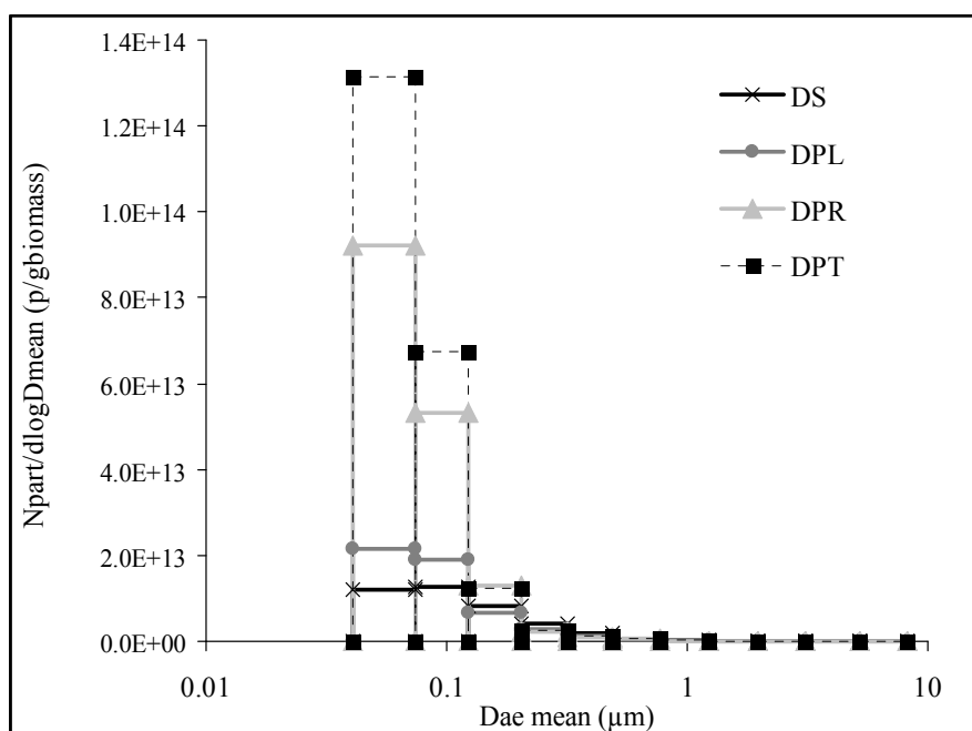
Fig. 6. Number size distributions of PM 10 for DPW at 800°C under an air flow rate of 50 NL/h.
