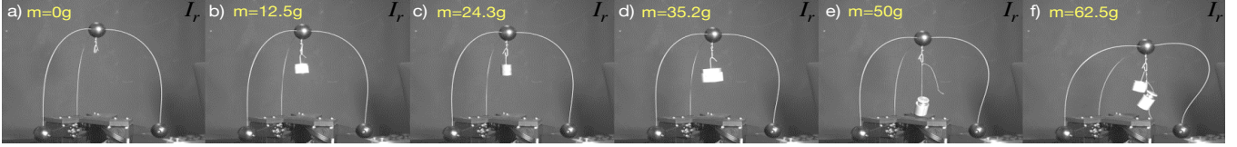
Fig. 12. Images of the different deformation configurations of the TriRod resulting by attaching weights ranging from 0g to 62.5g. The weights are attached to the centre sphere C .
