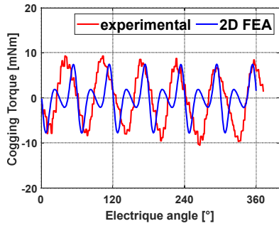
Fig. 16. Cogging torque waveforms.
