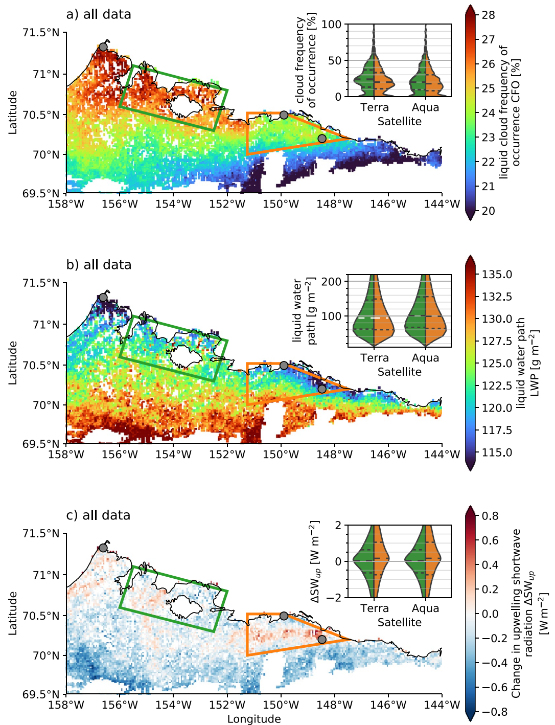
Figure 4. Spatial patterns of Moderate Resolution Imaging Spectroradiometer (MODIS) products showing (a) liquid containing cloud frequency of occurrence (CFO), (b) mean liquid water path (LWP), and (c) change in shortwave upwelling radiation \Delta\text{SW}_{\uparrow} with respect to the reference region (green box). The embedded violin plots show the underlying normalized distributions for the study (orange) and reference (green) region with the lines representing the median as well as the 25th and 75th percentiles. Note that for CFO and \Delta\text{SW}_{\uparrow} , the distribution of monthly values is shown and the full (i.e., non averaged) data set is shown for LWP. Median values colored in black indicate a significant difference (5% confidence interval) between the medians of the two regions. The gray circles indicate (from left to right) Utqiagvik, Oliktok Point, and Deadhorse; black lines show shorelines.
