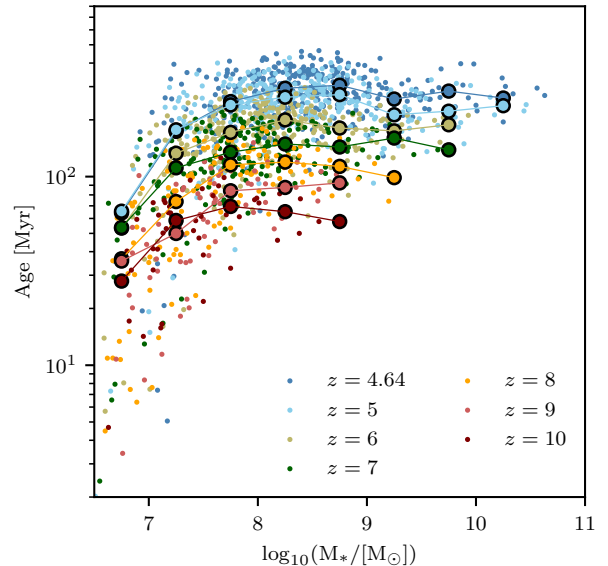
FIG. 9.— Mass-weighted stellar age in SPHINX for different redshifts as a function of galaxy stellar mass. The solid lines and large data points indicate the mean values while smaller data points show individual galaxies.
