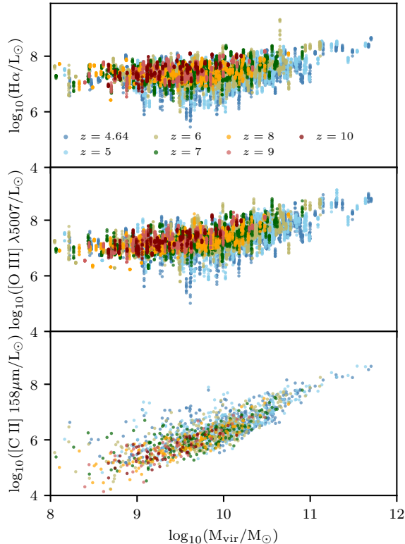
FIG. 28.— Observed H\alpha (top), [O\ III]\ \lambda 5007 (middle), and [C\ II]\ 158\mu\text{m} (bottom) emission versus halo virial mass. Because [C\ II]\ 158\mu\text{m} is not impacted by dust, we show only the intrinsic value of the emission line as it is the same across all ten sight lines.
