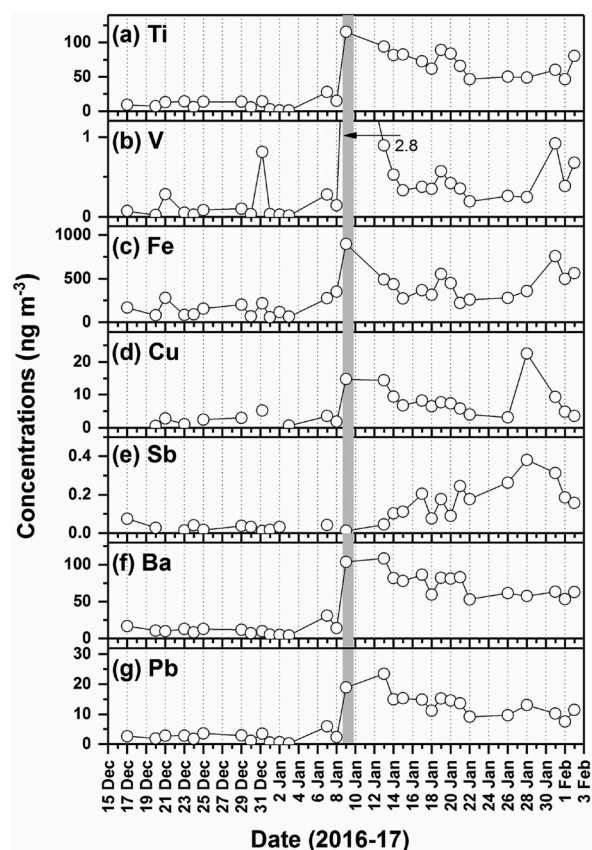
Fig. 7. Temporal variations of major trace metal species in \text{PM}_{10} aerosols at Bharati. The shaded line divides the whole sampling period into two parts such as high altitude Tropospheric aerosols (HTAs) and low altitude tropospheric aerosols (LTAs) aerosols.
