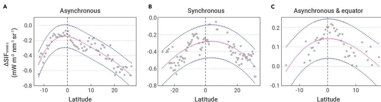
Figure 4. Latitudinal variation in \Delta SIF_{GOME-2} for the asynchronous (A, yellow in Figure 3), synchronous (B, blue in Figure 3), and asynchronous equatorial (C, purple in Figure 3) regimes. Note the unique vertical scale in (C). Black symbols are mean values for 0.5^\circ -latitude bands. Red lines were fitted using generalized additive models, and blue lines represent the 95% confidence intervals. SIF_{GOME-2} is solar-induced fluorescence. \Delta SIF_{GOME-2} equals the difference in mean SIF_{GOME-2} between dry and wet months (see supplemental methods for definition of dry and wet months).
