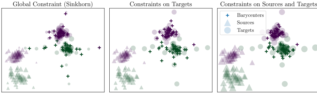
Figure 2: Toy domain adaptation scenario with entropic OT plans ( \xi = 10 ) with various constraints. The size of the point is proportional to the associated entropy. When using Sinkhorn, barycentric mapping match outlier points since the OT plan is less diffuse for these points. In turn, using pointwise constraints concentrate the mapped points in high-density regions, thus giving more robust estimates for the mappings onto the target domain.
