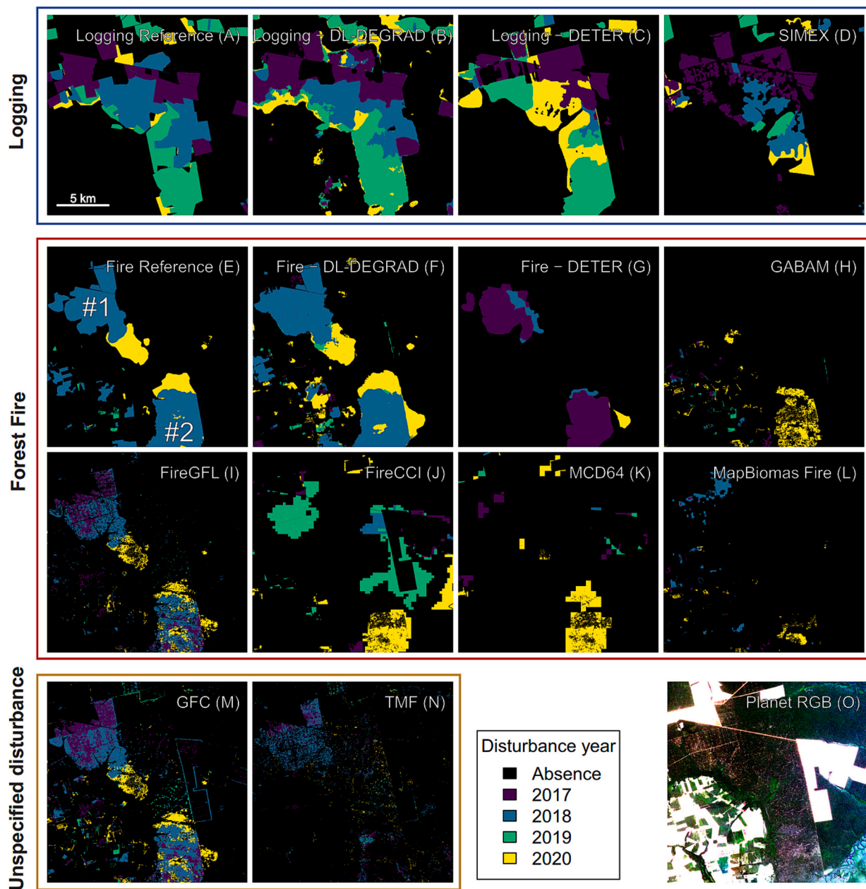
Fig. 4. Examples of cumulative forest degradation maps from the DL-DEGRAD and available products from 2017 to 2020 for a site located at 54° 14'W; 12° 7'S. (A-D) Logging mapped by the independent test dataset, DL-DEGRAD Logging, DETER Logging, and SIMEX, respectively. (E-L) Forest fire mapped by the independent test dataset, DL-DEGRAD Fire, DETER Fire, GABAM, FireGFL, FireCCI, MCD64, and MapBiomass Fire, respectively. (M-N) Unspecified Forest disturbances mapped by the GFC and TMF. (O) Planet NICFI true color composite from June 2020.
