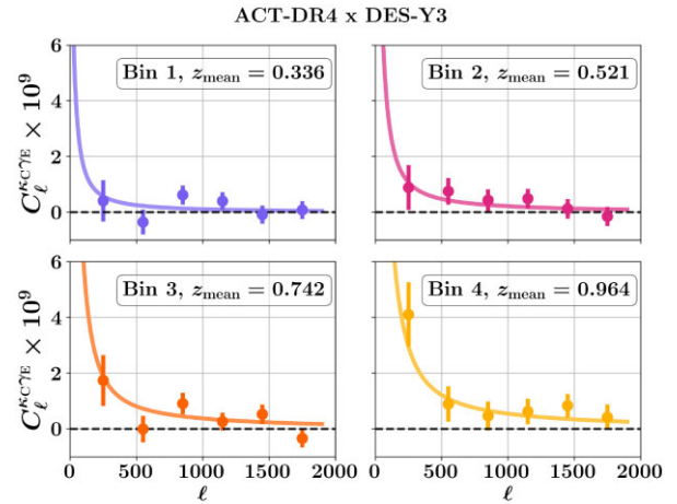
Figure A1. Similar to Section 7, but for ACT-only \kappa_{\text{C}} . The points with the error bar show C_\ell^{\kappa_{\text{C}}^{\text{C}/\text{YE}}} bandpowers with ACT-DR4 \kappa_{\text{C}} and DES-Y3 shear for four DES-Y3 redshift bins. Error bars are the square root of the diagonal of the covariance matrix. z_{\text{mean}} is the mean redshift of the source galaxy distribution. The curves show the best fit theory C_\ell^{\kappa_{\text{C}}^{\text{C}/\text{YE}}} .
