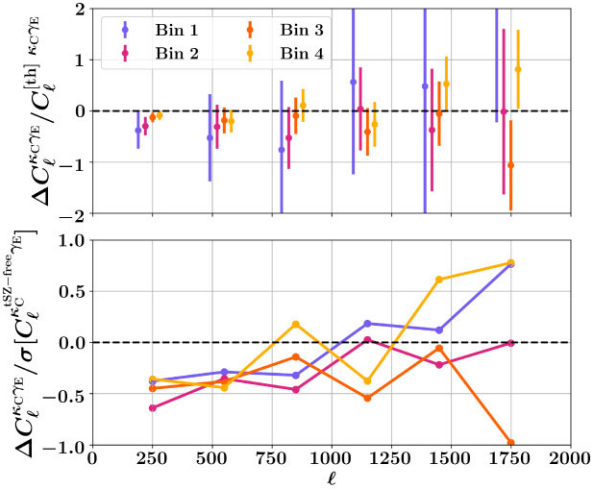
Figure A3. Comparison of C_\ell^{kC^{\gamma E}} [ACT-only, with-tSZ] and C_\ell^{kC^{\gamma E}} [ACT+ Planck , tSZ-free]. Top: The difference between two ( \Delta C_\ell^{kC^{\gamma E}} \equiv C_\ell^{\text{with-tSZ}} - C_\ell^{\text{tSZ-free}} ) relative to the fiducial theory C_\ell^{kC^{\gamma E}} . The error bars depict \sigma(\Delta C_\ell^{kC^{\gamma E}})/C_\ell^{[\text{th}]kC^{\gamma E}} , where \sigma(\Delta C_\ell^{kC^{\gamma E}}) is uncertainty on \Delta C_\ell^{kC^{\gamma E}} . Bottom: The same difference as in the top panel, \Delta C_\ell^{kC^{\gamma E}} , but now in units of error bar on tSZ-free C_\ell^{kC^{\gamma E}} .
