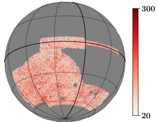
Figure 4. The source galaxy number density map in \text{gal}/\text{arcmin}^2 unit (top) and the weight map (bottom) for the galaxies in DES-Y3 Bin-4. For the weight map, the value in each pixel is the summation of the inverse variance weights of all the galaxies that fall within that pixel. The weight map is used as the shear field mask without apodization.
