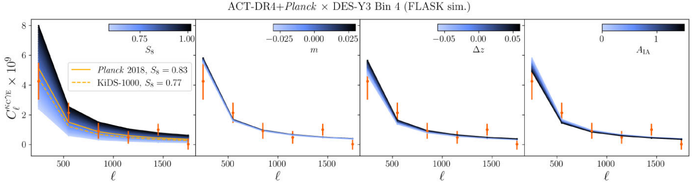
Figure 9. Illustrative changes in predicted data vectors as the cosmological and nuisance parameters are individually varied, compared to the simulated data vector described in Section 4.1 (to be concise, we only show tomographic Bin 4 as this is the highest SNR bin). The left-most panel also shows cosmologies with S_8 as found by Planck 2018 primary CMB (Planck Collaboration 2020) and the KiDS-1000+BOSS+2dFLENs galaxy clustering and weak lensing survey (Heymans et al. 2021) as examples of the range of values present in the current literature.
