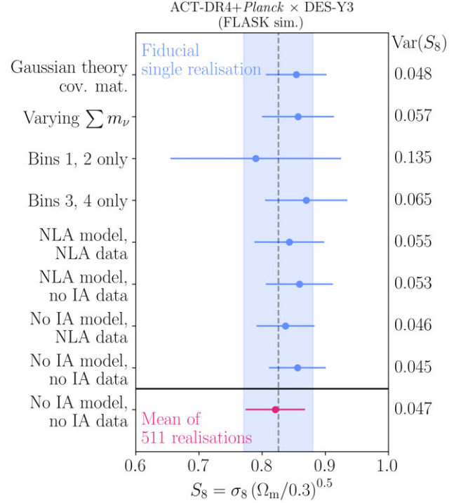
Figure 12. The stability of the recovery of the S_8 parameter from our simulated data vector as we change the model used for the inference. The dashed vertical line represents the true value of the input to the simulation, and the shaded band is the error bar in the fiducial model setup. Note that the slightly (but not significantly) high value recovered in the upper rows is consistent with what is expected for this single realization (see Fig. 14). The final row shows the result for one model using a data vector which is the mean of 511 realisations.
