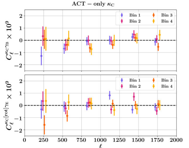
Figure A2. Similar to Fig. 10, but for ACT-only data. Top: The power spectrum between \kappa_{\text{C}} and the B-mode of the shear ( C_\ell^{\kappa_{\text{C}}^{\text{B}}} ), which is expected to be consistent with zero. Bottom: The correlation between \kappa_{\text{C}} and the E-mode of the shear map ( C_\ell^{\kappa_{\text{C}}^{\text{rot}^{\text{Y}^{\text{E}}}} ) obtained from the catalogue in which ellipticities are randomly rotated.
