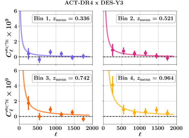
Figure A1. Similar to Section 7, but for ACT-only \kappa_{\text{C}} . The points with the error bar show C_\ell^{\kappa_{\text{C}}^{\text{C}^{\text{Y}^{\text{E}}}} bandpowers with ACT-DR4 \kappa_{\text{C}} and DES-Y3 shear for four DES-Y3 redshift bins. Error bars are the square root of the diagonal of the covariance matrix. z_{\text{mean}} is the mean redshift of the source galaxy distribution. The curves show the best fit theory C_\ell^{\kappa_{\text{C}}^{\text{C}^{\text{Y}^{\text{E}}}} .
