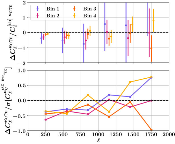
Figure A3. Comparison of C_\ell^{kC\gamma E} [ACT-only, with-tSZ] and C_\ell^{kC\gamma E} [ACT+ Planck , tSZ-free]. Top: The difference between two ( \Delta C_\ell^{kC\gamma E} \equiv C_\ell^{\text{with-tSZ}} - C_\ell^{\text{tSZ-free}} ) relative to the fiducial theory C_\ell^{kC\gamma E} . The error bars depict \sigma(\Delta C_\ell^{kC\gamma E})/C_\ell^{[th]kC\gamma E} , where \sigma(\Delta C_\ell^{kC\gamma E}) is uncertainty on \Delta C_\ell^{kC\gamma E} . Bottom: The same difference as in the top panel, \Delta C_\ell^{kC\gamma E} , but now in units of error bar on tSZ-free C_\ell^{kC\gamma E} .
