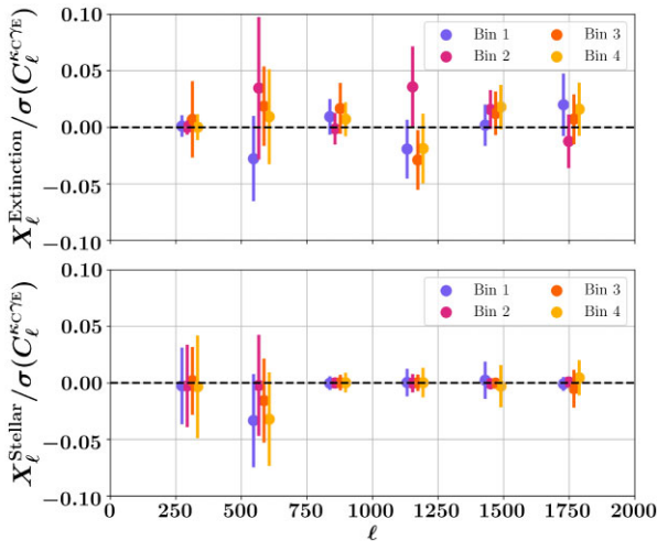
Figure 11. Survey property correlation statistics X_\ell in units of error bar of C_\ell^{KCYE} , for the dust extinction map (top panel) and the stellar density (bottom panel). The error bars are obtained using X_\ell computed over 28 jackknife samples of the data. For both survey properties, X_\ell^S is less than 5 per cent of the error bar on C_\ell^{KCYE} and consistent with zero.
