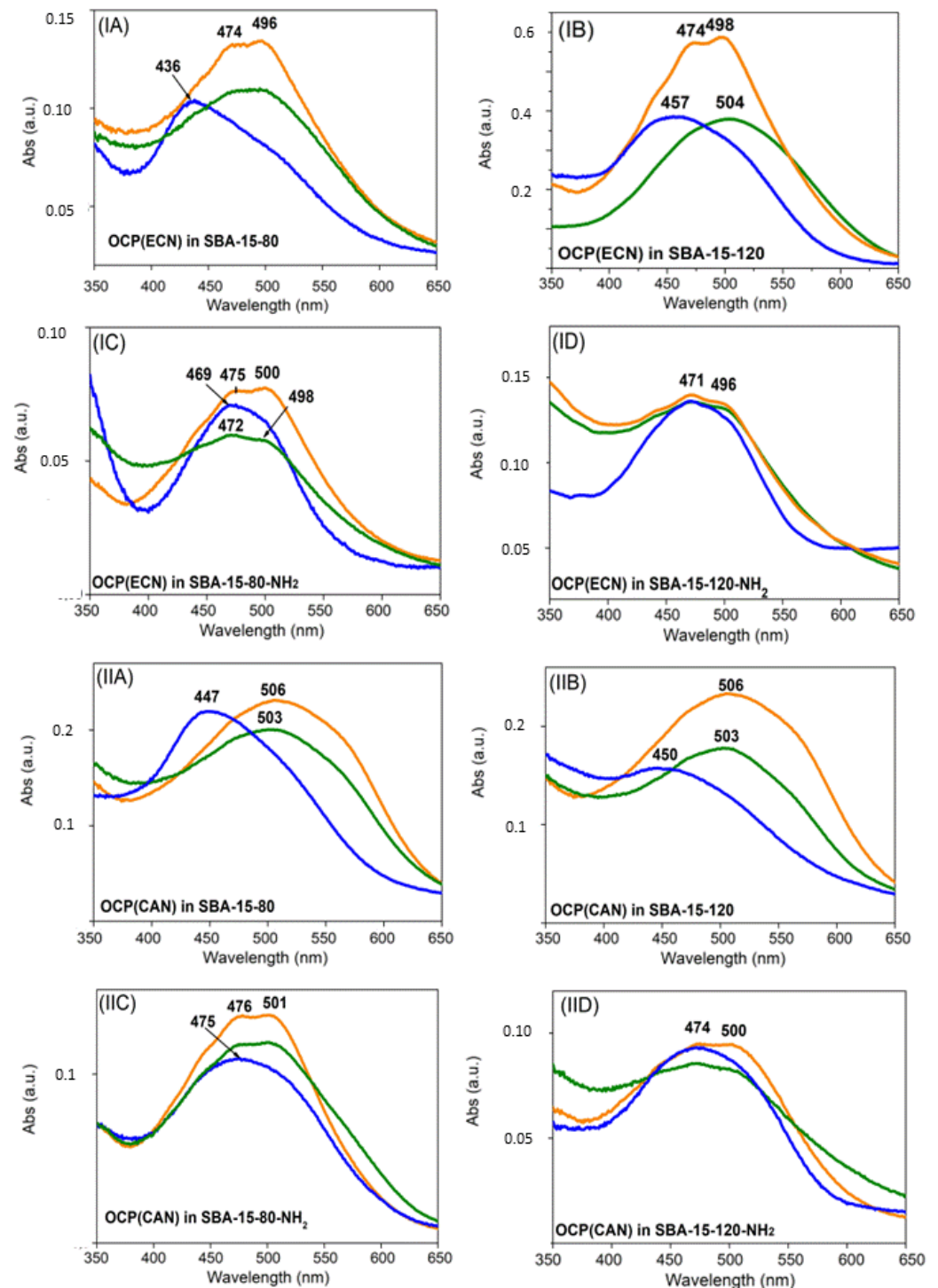
Figure 7. OCP(ECN) in SBA-15-80 (6 nm pore diameter) (IA); SBA-15-120 (8 nm pore diameter) (IB); SBA-15-80-NH 2 (IC); SBA-15-120-NH 2 (ID); OCP(CAN) in SBA-15-80 (IIA); SBA-15-120 (IIB); SBA-15-80-NH 2 (IIC); SBA-15-120-NH 2 (IID). Absorption visible spectra recorded in 350–700 nm range. (Orange) spectra recorded at room temperature before thermal treatment; (green) spectra of samples treated at 40 °C; (blue) spectra of samples treated at 60 °C. Spectral intensity variability depended on sample preparation before the analysis. Experiments were carried out as follows: the solid sample was heated to the desired temperature using temperature-controlled distilled water in a beaker for 30 min. Then a Vis spectrum of the sample was recorded. The whole procedure was carried out in darkness to avoid photo-activation of OCP.
