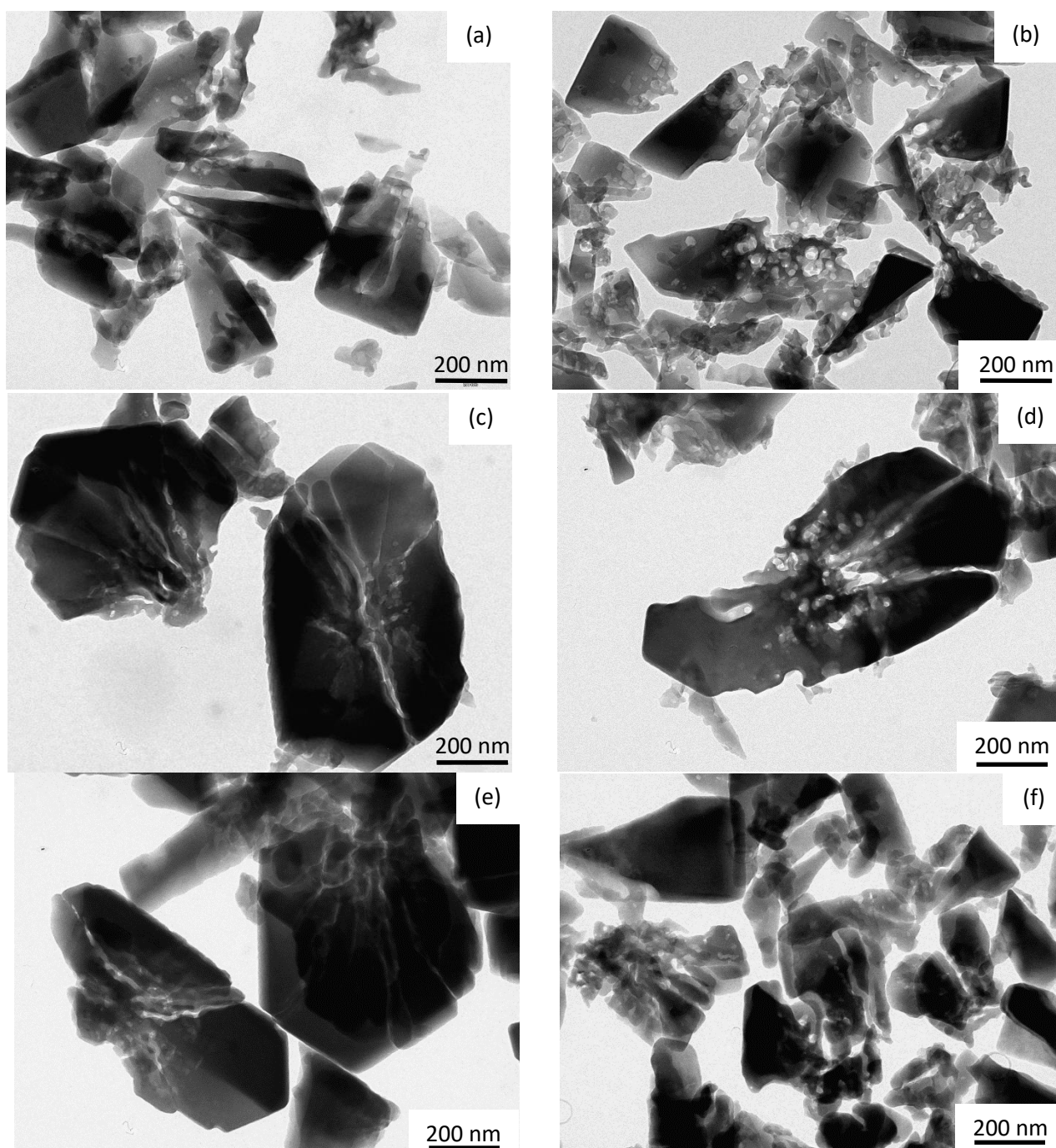
Figure 5 : TEM monitoring of the dissolution of 1 (a, b), 2 (c, d), and 4g \text{NH}_4\text{-ZSM-5} (e, f) in 20 g of 40 wt% of \text{NH}_4\text{F} solution for 1h (a, c, e) and 2h (b, d and f)
