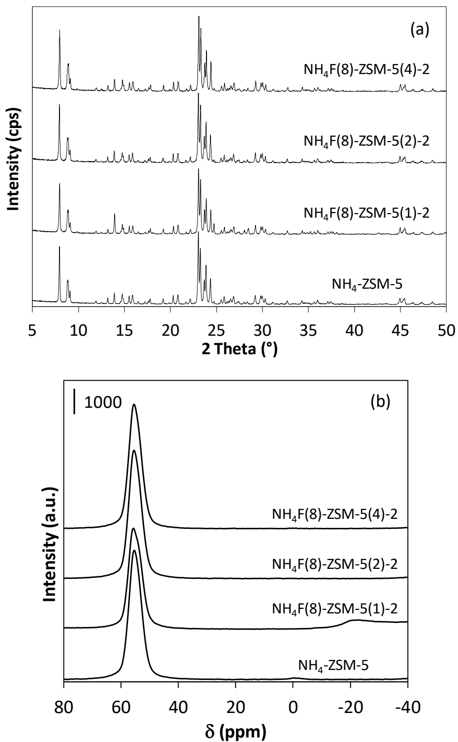
Figure 1: Impact of solid:liquid ratio on the zeolite structure characteristics: (a) XRD patterns and (b) ^{27}\text{Al} MAS NMR spectra of the parent \text{NH}_4\text{-ZSM-5} and samples etched 2 h in a 40 wt% \text{NH}_4\text{F} solution.
