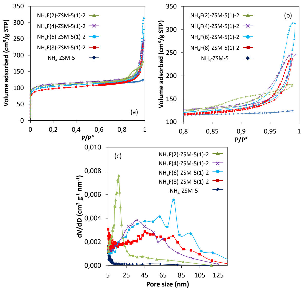
Figure 7: (a, b) \text{N}_2 adsorption isotherms and (c) BJH pore size distributions of the parent \text{NH}_4\text{-ZSM-5} and the samples etched in a solution containing from 8 to 2 g of \text{NH}_4\text{F} and 12 g of water. Amount of zeolite used: 1 g.
