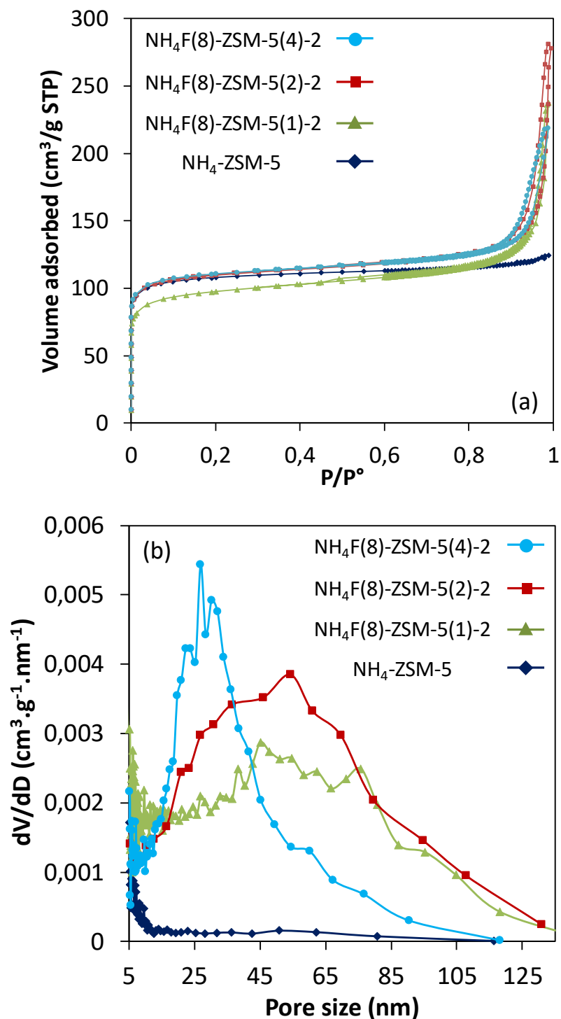
Figure 2: (a) N_2 adsorption isotherms and (b) BJH pore size distributions of the parent NH_4 -ZSM-5 and of samples etched 2 h in a 40 wt% NH_4F solution.
