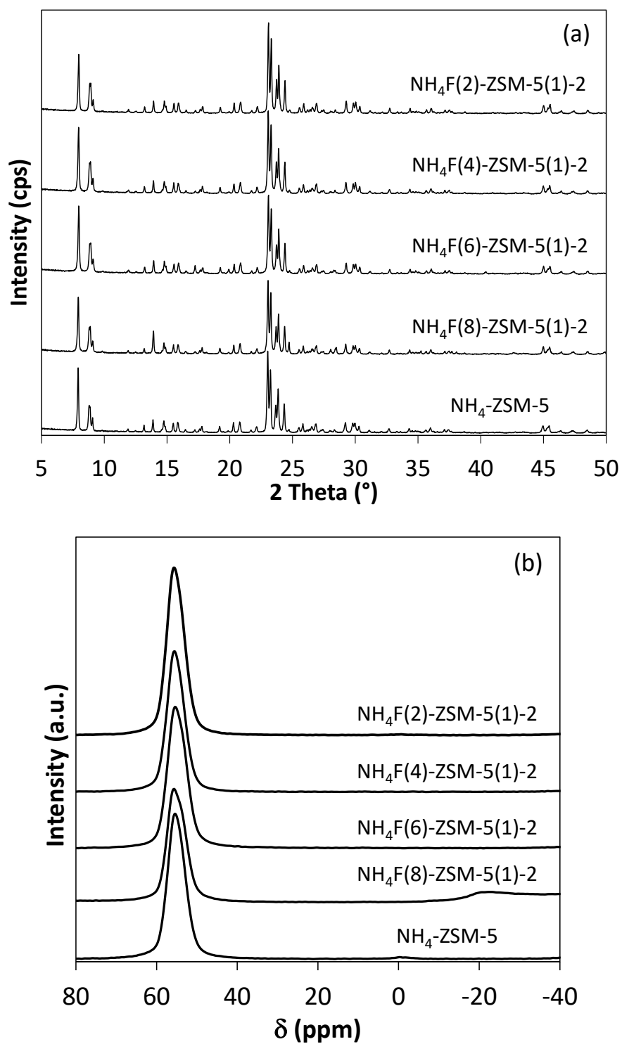
Figure 6: (a) XRD patterns and (b) ^{27}\text{Al} MAS NMR spectra of the parent \text{NH}_4\text{-ZSM-5} and of samples etched 2 h in a solution containing from 8 to 2 g of \text{NH}_4\text{F} and 12g of water. Amount of zeolite used: 1 g.
