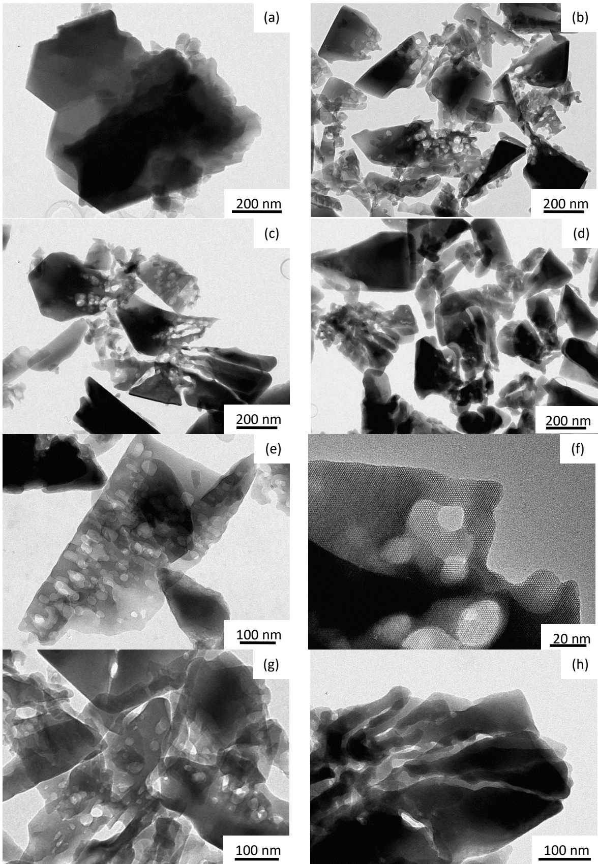
Figure 3: TEM monitoring of the dissolution of MFI as function of the amount of zeolite treated in 20 g of 40 wt% of \text{NH}_4\text{F} solution for 2h – (a) \text{NH}_4\text{-ZSM-5} ; (b, e, f) \text{NH}_4\text{F(8)-ZSM-5(1)-2} ; (c, g) \text{NH}_4\text{F(8)-ZSM-5(2)-2} ; (d, h) \text{NH}_4\text{F(8)-ZSM-5(4)-2}
