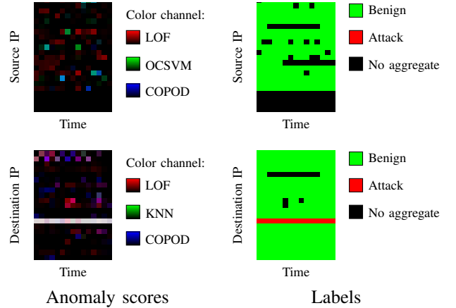
(b) Brute-force attack. In the label images, the victim is shown to receive but not emit attack flows. The attack is only visible in the destination IP address representation, where the UL models detect the entire attack line as highly anomalous, along with some weakly anomalous benign aggregates.
