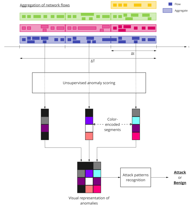
Fig. 4: Attack pattern recognition on a visual representation of the detected anomalies during a timeframe \Delta T . The timeframe \Delta T consists of, in this example, 3 consecutive time intervals \Delta t . The network flows from each time interval \Delta t are analyzed as shown in Figure 2. All the anomalies detected by the N = 3 base-learners within a specific time interval \Delta t are visually represented using color-coded segments. By arranging the 3 segments side by side, we obtain a visual representation of network anomalies detected by the N = 3 base-learners during the timeframe \Delta T .
