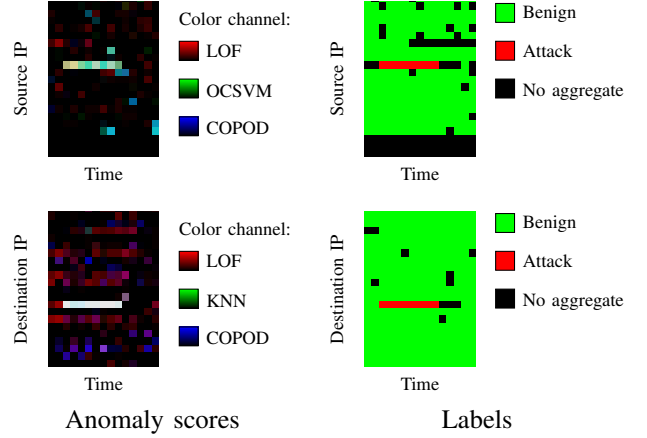
(a) DoS attack. In the label images, a red horizontal line indicates close emission and reception of attack flows by the victim. In the destination IP address representation, the UL models detect the entire attack line as highly anomalous, with some weakly anomalous benign aggregates. In the source IP address representation, the attack line is detected as moderately anomalous.
