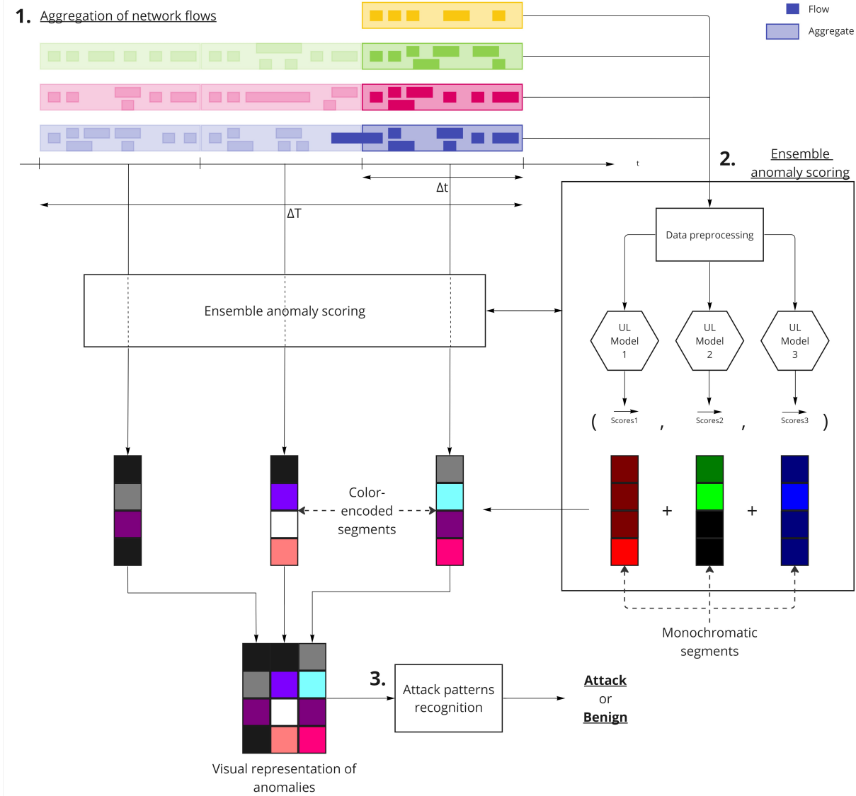
Fig. 1: System overview. The system analyzes a traffic capture over a period \Delta_T . First, it aggregates network flows from the capture that belong to the same time interval \Delta_t and computes their features. Next, it applies a set of three unsupervised base-learners to assign anomaly scores to the aggregates. After that, the system generates a visual representation of the detected anomalies, enabling a visualization of potential attack patterns. Finally, these representations are analyzed by an attack pattern recognition module, here a CNN, which determines whether the network is under attack during the period \Delta_T .
