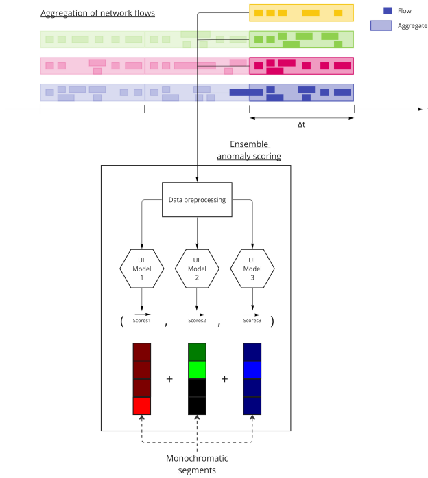
Fig. 2: Anomaly scoring by three unsupervised base-learners during a time interval \Delta_t . This analysis generates a vertical color-encoded segment that is part of the visual representation of anomalies generated in Figure 4. Four network flows are grouped into aggregates during a time interval \Delta_t . Then, the features of the aggregates are extracted and prepared before being evaluated by the three unsupervised base-learners. Each base-learner assigns an anomaly score to each aggregate. A color is assigned to each model, allowing the representation of anomaly scores on a monochromatic segment. By overlaying the monochromatic segments from the base-learners, we obtain a color-encoded segment that represents the anomalies detected by the set of base-learners.
