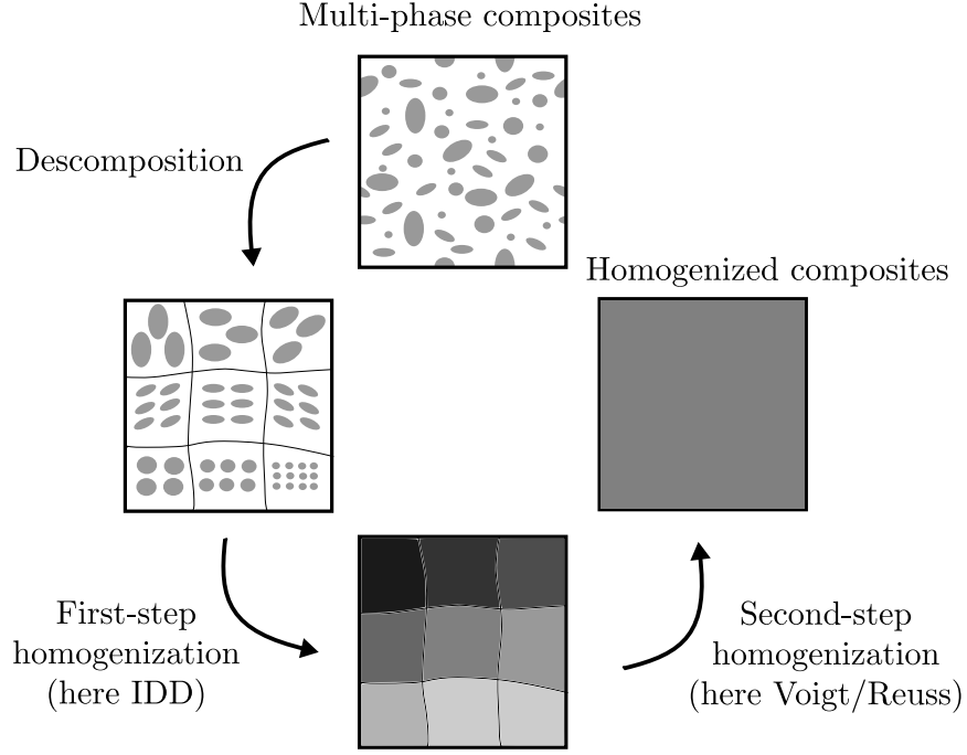
Figure 3: Two-step homogenization procedure.
