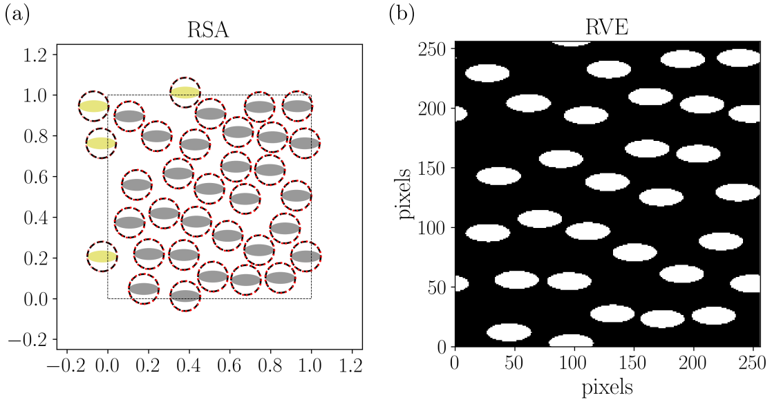
Figure 14: Circular RSA cells and elliptic inclusions: (a) RSA process. (b) 2D representative element of the microstructure.
