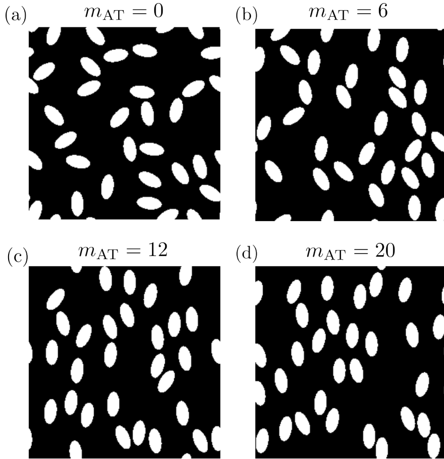
Figure 21: Elliptic inclusions with different orientations following the Advani-Tucker law: examples of RVE for four values of the parameter m_{\text{AT}} .
