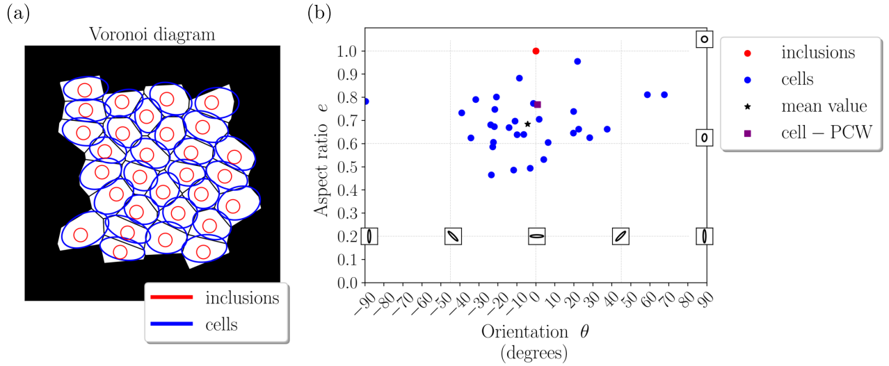
Figure 11: Elliptic RSA cells and identical inclusions (circular here): (a) Voronoï diagram, inclusions and respective cells. (b) Scatter plot between aspect ratio and orientation.
