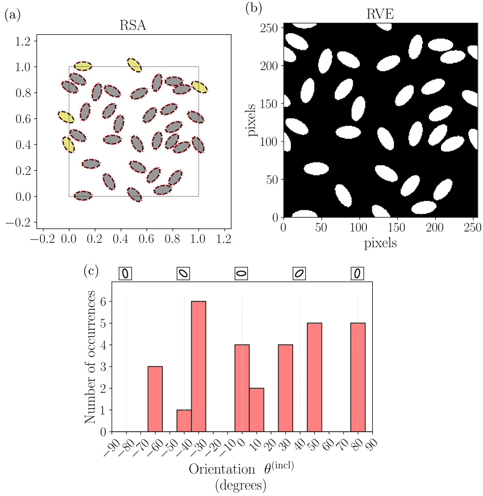
Figure 18: Elliptic inclusions with different orientations: (a) RSA process with RSA-cells coinciding with inclusions. (b) RVE of the microstructure. (c) Number of inclusions per chosen orientation.
