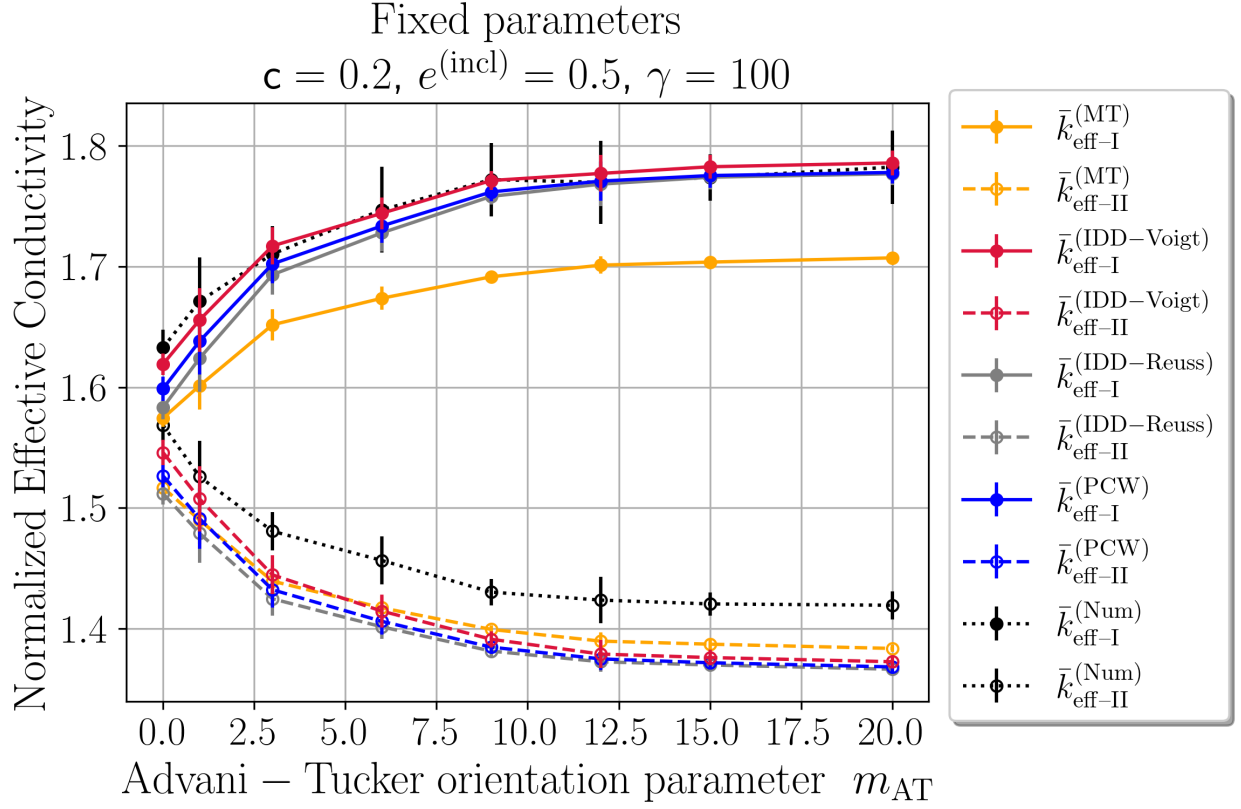
Figure 22: Elliptic inclusions with different orientations following the Advani-Tucker law: mean values and standard deviations of the normalized effective conductivity properties obtained using 10 microstructures for each value of the parameter m_{\text{AT}} .
