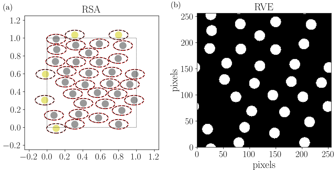
Figure 10: Elliptic RSA cells and identical inclusions (circular here): (a) RSA process (see Section 4.1.1) with the parameters of Table 3. (b) RVE of the 2D microstructure.
