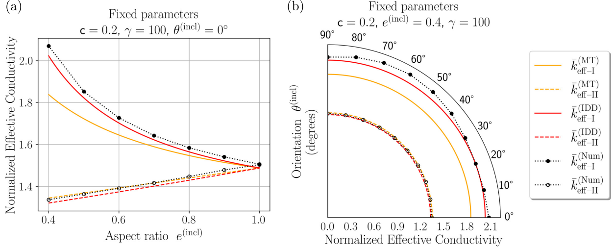
Figure 16: Circular RSA cells and elliptic inclusions: MT and IDD performance compared to the FF numerical approach for different aspect ratios and orientations of inclusions.
