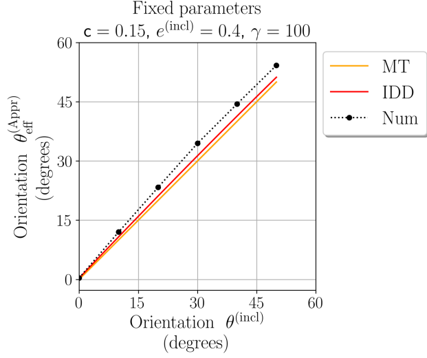
Figure 13: Elliptic RSA cells and identical elliptic inclusions: directions of anisotropy of the effective tensors, as a function of orientations of inclusions.
