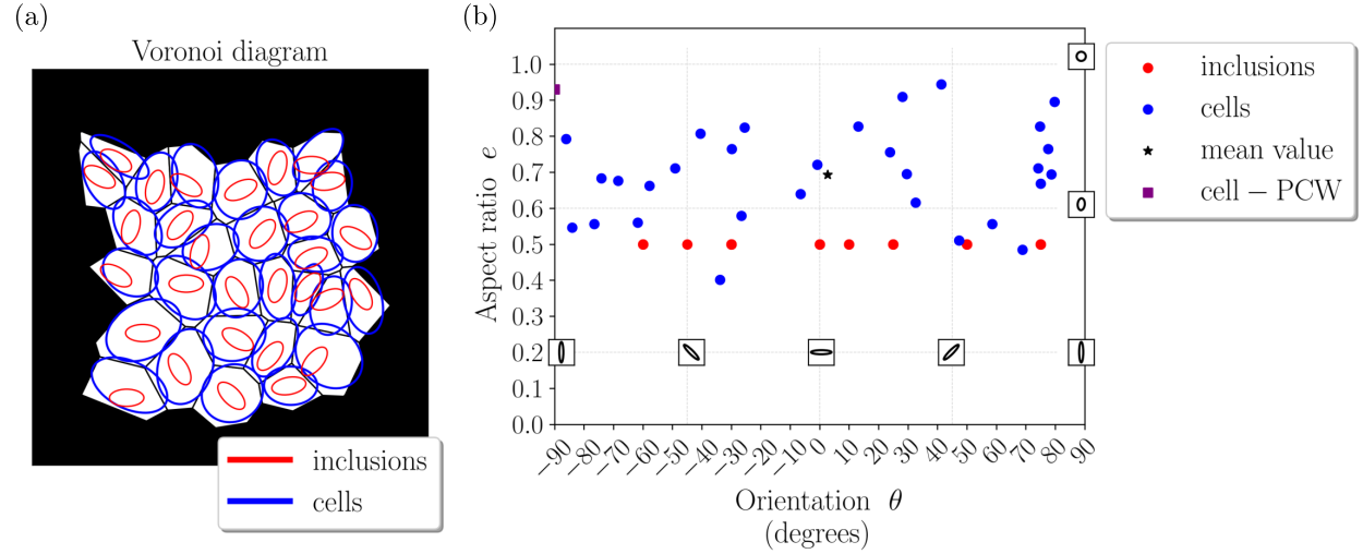
Figure 19: Elliptic inclusions with different orientations: (a) Voronoi diagram, inclusions and respective cells. (b) Scatter plot between aspect ratio and orientation.
