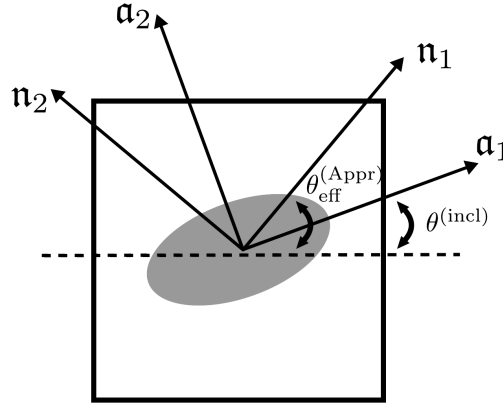
Figure 9: Notations for the orientations of inclusions and effective conductivity tensor.
