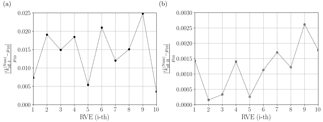
Figure C.24: Circular RSA cells and elliptic identical inclusions: relative difference between the effective conductivities of 10 RVE (parameters of Table 4) and their means over these 10 RVE, denoted by \mu_{10} . (a) k_{\text{eff-I}} and (b) k_{\text{eff-II}} .
