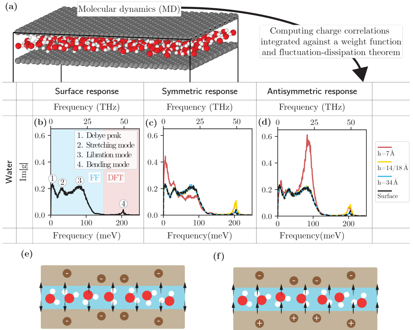
FIG. 3. Water response functions from simulation. a) Snapshot of a FF molecular dynamics simulation with 7 Å confinement b-d) Response functions \text{Im}[g(q, \omega)] of water as a function of the frequency \omega obtained from the simulations, at fixed wavevector q = 0.67 \text{ \AA}^{-1} for FF and q = 1 \text{ \AA}^{-1} for DFT. Different confinements are used: 7 Å, 14 Å (only FF), 18 Å (only DFT), 34 Å and 60 Å (only FF). b) Surface response function computed from simulations at weak confinement (FF at h=60 \text{ \AA} and DFT at h=34 \text{ \AA} ). c) Symmetric response function for different confinements. The dashed black line is the non-confined surface response function. d) Antisymmetric response function for different confinements. The dashed black line is the non-confined surface response function. e) Schematic of a channel containing a single water monolayer on which a symmetric potential is applied. f) Same as (e) with application of an antisymmetric potential.
