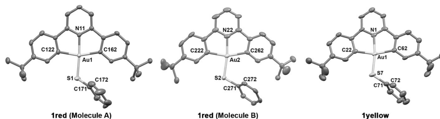
Figure 1. Structure of (C ^ N ^ PZ ^ ΔC)AuSPh ( 1 red ). [28] Ellipsoids set at 50% probability; H atoms omitted for clarity. Selected bond distances [Å] and angles [°]: Molecule A: Au1–S1 2.273(1), Au1–N11 2.006(3), Au1–C122 2.086(4), Au1–C162 2.091(4); N11–Au1–S1 175.66(8), C122–Au1–N11 80.5(1), C162–Au1–N11 80.6(1), C122–Au1–S1 95.46(9), C162–Au1–S1 103.38(9), Au1–S1–C171 110.2(2), torsion Au1–S1–C171–C172 50.1(4). Molecule B: Au2–S2 2.277(1), Au2–N21 2.017(4), Au2–C222 2.083(4); N21–Au2–S2 172.2(1), C222–Au2–N21 80.6(1), C262–Au2–N21 80.1(1), C222–Au2–S2 91.8(1), C262–Au2–S2 107.49(9), Au2–S2–C271 110.9(1), torsion Au2–S2–C271–C272 58.2(3). 1 yellow : Au1–S7 2.276(2), Au1–N1 2.022(6), Au1–C22 2.088(7), Au1–C62 2.080(7); N1–Au1–S7 170.94(18), C22–Au1–N1 81.3(3), C62–Au1–N1 79.8(3), C22–Au1–S7 89.6(2), C62–Au1–S7 109.2(2), Au1–S7–C71 116.6(3), torsion Au1–S7–C71–C72 94.3(6).
