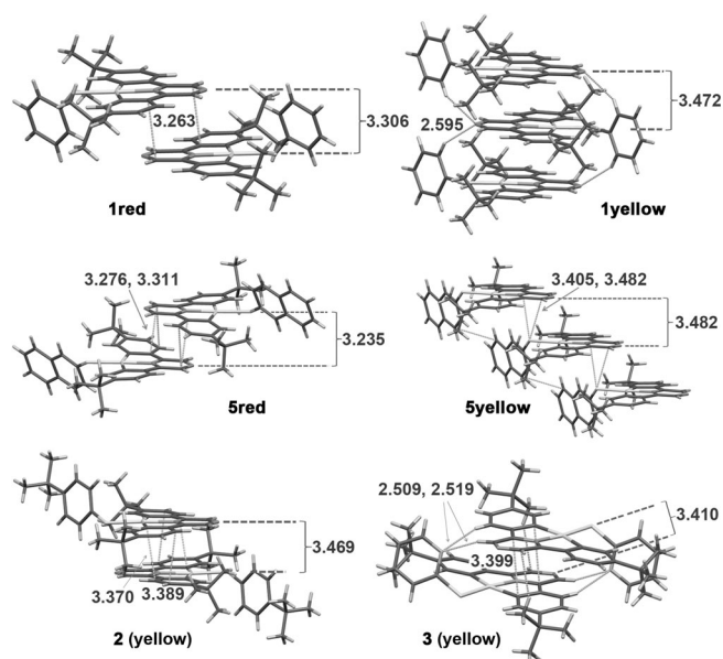
Figure 3. Intermolecular packing in emissive (red) and non-emissive (yellow) polymorphs of gold(III) thiolates, showing the pz...pz stacking of the red and pz...Au–S alignment of the yellow forms (pz = pyrazine). The inter-plane distance is measured between coordination planes of Au defined by Au, N, and C (bonded to Au). The packing diagrams of 1 yellow and 3 also show \text{CH}\cdots\text{N} close contacts ( <2.6 Å).
