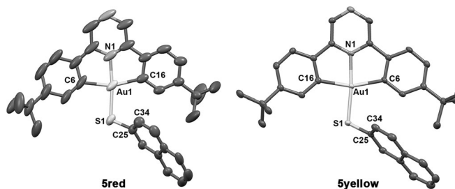
Figure 2. Left: Structure of (C ^ N ^ PZ ^ ΔC)AuSNp-2 ( 5 red ). [28] Ellipsoids set at 50% probability; H atoms omitted for clarity. Selected bond distances [Å] and angles [°]: Au1–S1 2.263(2), Au1–N1 2.006(6), Au1–C6 2.069(6), Au1–C16 2.080(6); N1–Au1–S1 174.3(2), C6–Au1–N1 80.6(3), C16–Au1–N1 80.1(2), C6–Au1–S1 93.8(2), C16–Au1–S1 105.6(2), Au1–S1–C25 109.5(2), torsion Au1–S1–C25–C34 52.3(5). Right: 5 yellow : Au1–S1 2.2837(8), Au1–N1 2.014(3), Au1–C6 2.095(3), Au1–C16 2.086(3); N1–Au1–S1 174.05(7), C6–Au1–N1 80.7(1), C16–Au1–N1 80.2(1), C6–Au1–S1 104.68(8), C16–Au1–S1 94.53(8), Au1–S1–C25 109.8(1), torsion Au1–S1–C25–C34 56.5(3).
