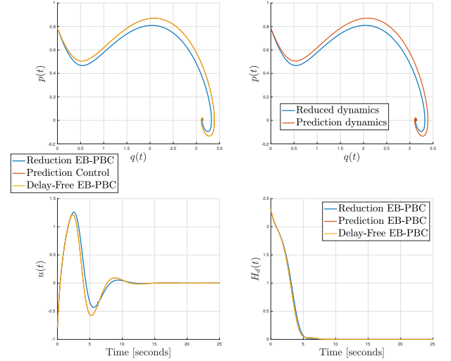
Fig. 1. The retarded pendulum with \delta = \tau = 5 \times 10^{-4} .
