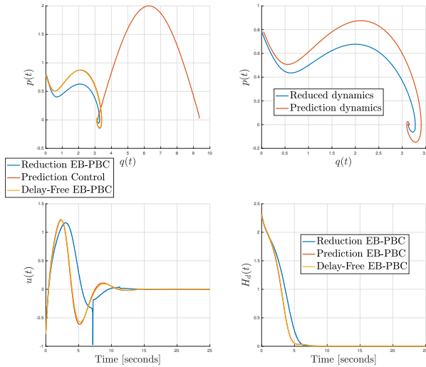
Fig. 2. The retarded pendulum with \delta = \tau = 5 \times 10^{-2} .
