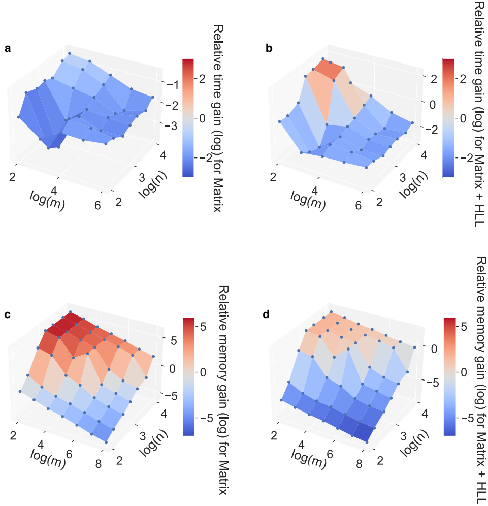
Figure 3: Fraction of computational time (top row) and memory usage (bottom row) of the component matrix methods divided by the ones of the EG+HLL method. Panels (a) and (c) depict results for the exact component matrix method, while panels (b) and (d) are for its approximate solution using HLL. All scales are logarithmic with colour blue indicating when the component matrix method performs better (and red in the contrary case).
