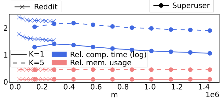
Figure 7: Relative computation time and relative memory usage for the Reddit and Superuser datasets to compute the distribution of the largest out-components thanks to the hashing framework compared to the matrix method depending on the number of events m .
