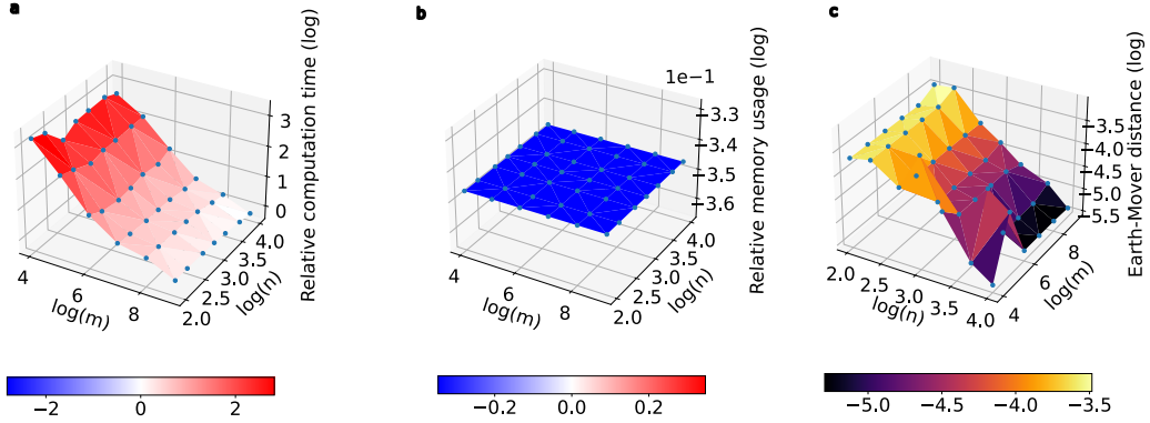
Figure 5: a) Relative time and b) relative memory usage for the computation of the distribution of the largest out-components compared to the ground-truth given by the matrix method on synthetic data. c) Accuracy of the hashing framework given by the Earth-Mover distance.
