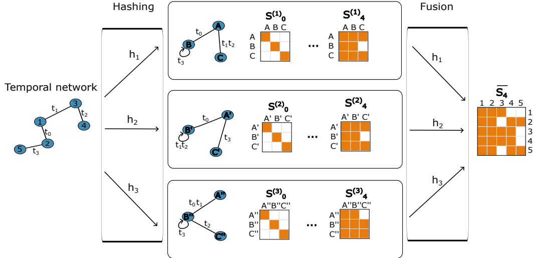
Figure 4: From a 5 nodes temporal network, several hashed version are computed with 3 nodes each. Then, every hashed graph can be used to compute a small component matrix thanks to our matrix algorithm. Finally, the different component matrices can be fused to compute an approximate solution of the component matrix of the initial temporal network.
