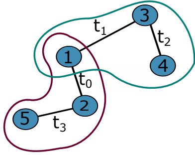
Figure 1: Left: a temporal network defined as a series of events ordered in time ( t_i < t_j for i < j ). The out-component of node 3 is circled in blue; the in-component of node 2 is circled in purple. Right: the corresponding component matrix. A row depicts the in-component of a node (we emphasise that of node 2). A column depicts the out-component of a node (we emphasise that of node 3): a non-zero element in the u -th column at coordinate v , means that node v belongs to the out-component of node u .
