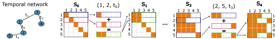
Figure 2: From a given temporal network (left graph), we compute the Component Matrix (right matrix) of size n \times n , with n = 5 , by scanning the series of events. For each event, we compute the OR operation between the rows of the matrix corresponding to the interacting nodes and replace them by the result. Matrix S_4 is the component matrix at the end of the streaming after m = 4 events.
