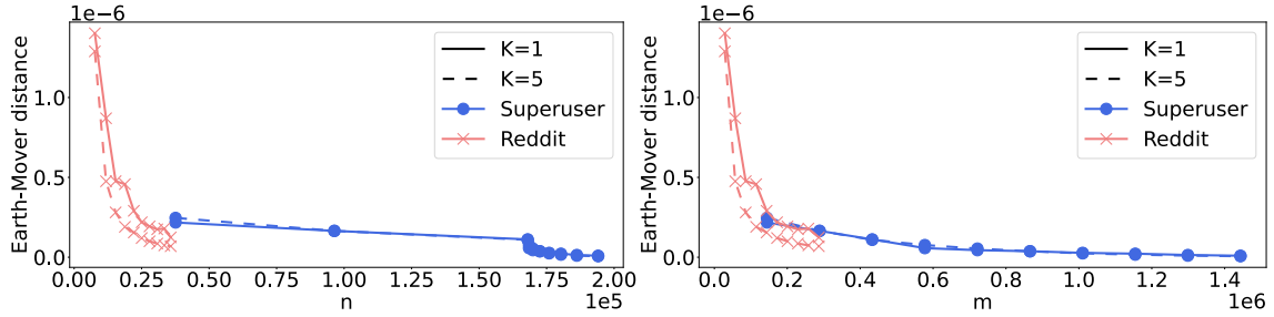
Figure 8: Accuracy for the Reddit dataset and the Superuser dataset to compute the distribution of the largest out-components thanks to the hashing framework compared to the matrix method.
