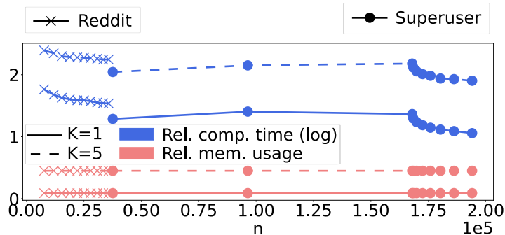
Figure 6: Relative computation time and relative memory usage for the Reddit and Superuser datasets to compute the distribution of the largest out-components thanks to the hashing framework compared to the matrix method depending on the number of nodes n .
