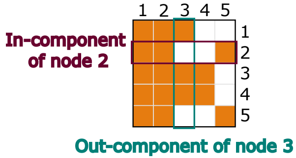
Figure 1: Left: a temporal network defined as a series of events ordered in time ( t_i < t_j for i < j ). The out-component of node 3 is circled in blue; the in-component of node 2 is circled in purple. Right: the corresponding component matrix. A row depicts the in-component of a node (we emphasise that of node 2). A column depicts the out-component of a node (we emphasise that of node 3): a non-zero element in the u -th column at coordinate v , means that node v belongs to the out-component of node u .
