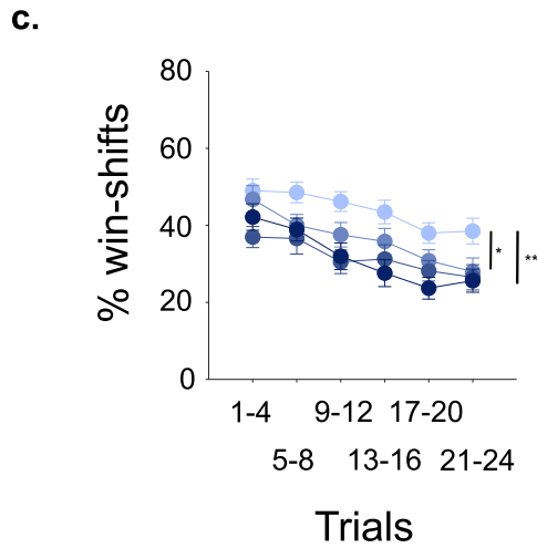
Figure 2: Between session changes in behaviour. a. & b. Mean performance +/- s.e.m. (n=24 subjects) increases between sessions in low- and high-risk blocks respectively. Stars indicate that for a given trial performance is significantly different between at least two groups of sessions. c. & d. Mean win-shift +/- s.e.m. decreases between sessions in low- and high-risk blocks respectively. Because of the lack of a significant interaction trial x sessions x risk, win-shift is not compared trial by trial as with performance but over all low- or high-risk blocks of different sessions. Significance levels as follows: * : p < 0.05 ; ** : p < 0.01 , *** : p < 0.001 .
