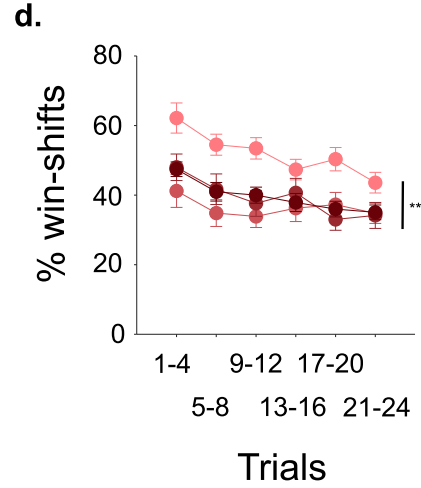
Figure 2: Between session changes in behaviour. a. & b. Mean performance +/- s.e.m. (n=24 subjects) increases between sessions in low- and high-risk blocks respectively. Stars indicate that for a given trial performance is significantly different between at least two groups of sessions. c. & d. Mean win-shift +/- s.e.m. decreases between sessions in low- and high-risk blocks respectively. Because of the lack of a significant interaction trial x sessions x risk, win-shift is not compared trial by trial as with performance but over all low- or high-risk blocks of different sessions. Significance levels as follows: * : p < 0.05 ; ** : p < 0.01 , *** : p < 0.001 .
