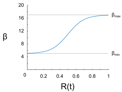
Figure 5: Regulation mechanisms of the inverse temperature in the different models.
