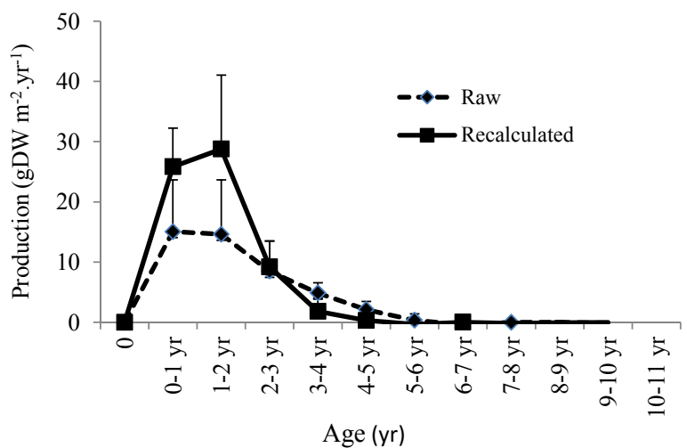
Figure 6. Average annual production (g shell-free DW.m 2 .yr -1 , + 1 standard deviation) per age of Crepidula fornicata from “raw” and “recalculated” database.
