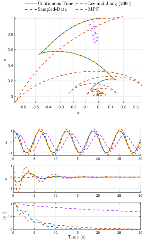
Fig. 1: Steering at the origin with \delta = 0.1 seconds.
