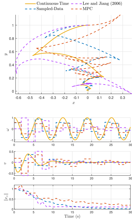
Fig. 2: Steering at the origin with \delta = 1.8 seconds.
