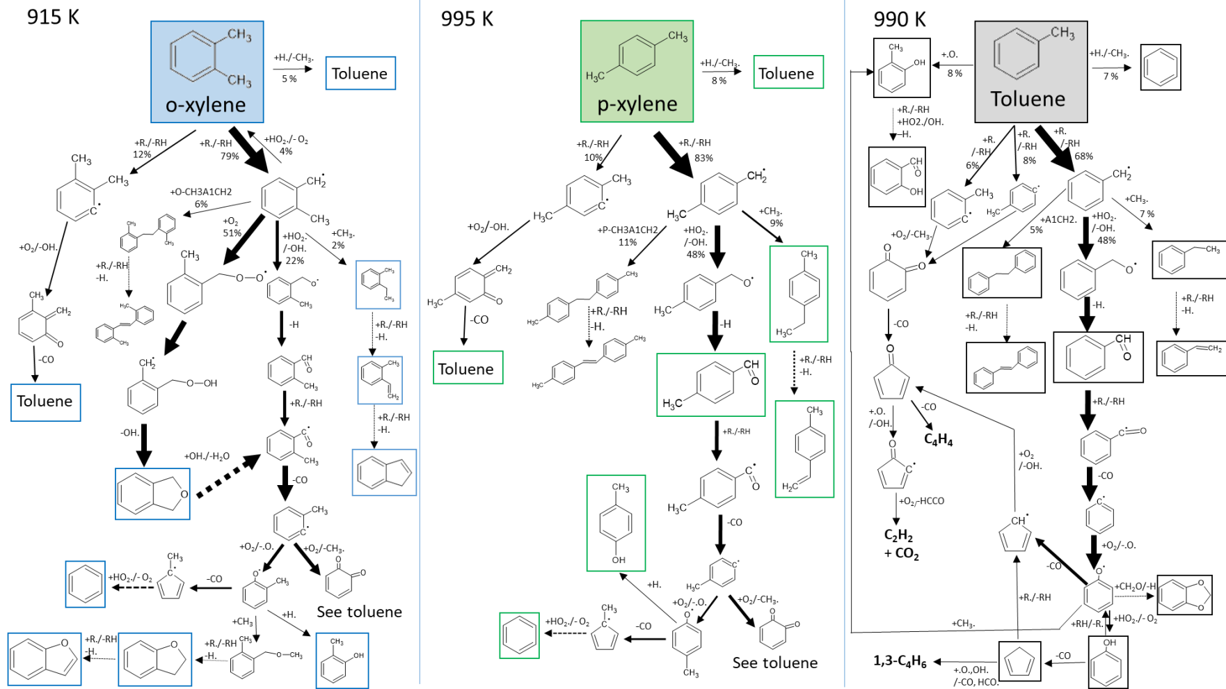
Figure 6: Flow-rate analyses during the oxidation of toluene, o-xylene, and p-xylene (same as m-xylene). Fuel conversion of 50%, \varphi = 1 .
