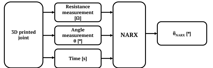
Fig. 13: Inputs and output for the proposed NARX neural network model, which the bending angle estimated by this model is denoted as \hat{\theta}_{NARX} .
