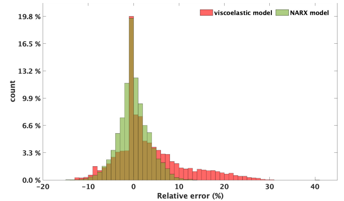
Fig. 22: Histogram of normalized data errors of both viscoelastic and NARX models.
