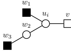
Figure 5: Vertex v is adjacent to a 3-worse-vertex.
