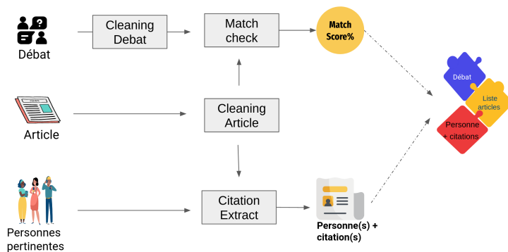
Figure 3: Final workflow proposed
