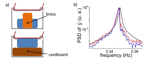
FIG. 4. (Color online) a) A piece of brass or cardboard is inserted in the envelope to change the total mass and mass geometry. b) Close view of the fundamental peak of FFT power density spectrum of \ddot{y} : smartphone alone (black), smartphone and brass piece (red), smartphone lifted up by a cardboard piece (blue). The slight decrease in frequency, is attributed to the elongation of the threads after the heavy brass piece has been inserted.
