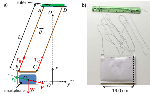
FIG. 1. (Color online) a) sketch and b) picture of our pendulum. The smartphone is inserted in an envelope suspended by two parallel 2 m-long almost inextensible threads. These threads are wound on a ruler to allow both precise geometry and easy clamping onto a building beam. The smartphone's overall motion is circular, but the body does not rotate around its center of mass. The envelope orientation remains parallel to its orientation at rest: each point within the envelope follows a circular path with radius L , but each with a different center e. g. A for B , D for C and O' for G .
