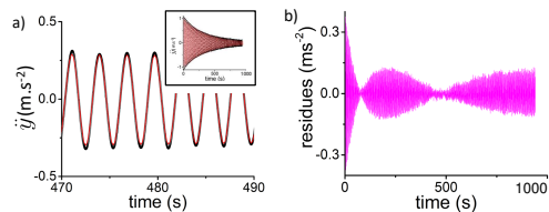
FIG. 5. (Color online) a) A few periods around 480 s: raw data (black dots) and damped sine fit (red line). Inset: full record. Agreement seems quite satisfactory. b) Residuals from the fit showing a large and structured discrepancy between the data and the fitted curve.
