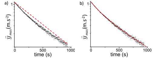
FIG. 7. (Color online) a) Maximum of the absolute value of the acceleration for each half period (black dots, in log-scale). Exponential decay, as predicted by the damped harmonic oscillator model, would produce a linearly decreasing amplitude (red dashed line) which is obviously not the case. b) Numerical simulations, discussed in more detail in the Supplementary Material 23 : data is quite well reproduced by an almost equal contribution of viscous and aerodynamic damping (red line).
