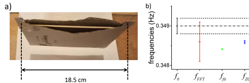
FIG. 2. (Color online) a) Picture showing the slight deformation when the smartphone is inserted despite the wooden stick inserted to stiffen the envelope. b) Comparison of the different values of the pseudo-frequency as determined by: f_0 (black: damped harmonic oscillator model), f_{FFT} (red: FFT of the recorded data points), f_{fit} (green: damped sine wave fit), f_{ZC} (blue: zero-crossing times linear regression). The residual plot (Fig. 6b) shows that the explanation for this inconsistency is the variation of the frequency over time.
