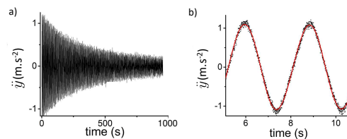
FIG. 3. (Color online) a) Raw data b) first few seconds of the record showing oversampling of the data allowing strong noise reduction through low pass filtering (red line).
