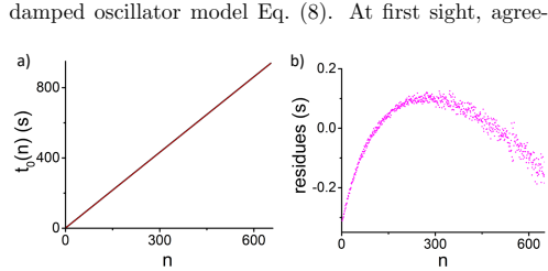
FIG. 6. (Color online) a) t_0(n) are the zero-crossing times of \ddot{y} successively numbered by n (black points). Red line: linear adjustment hardly distinguished from data points. b) Residual plot showing that the oscillation period is not constant, but has a regular variation over time.
