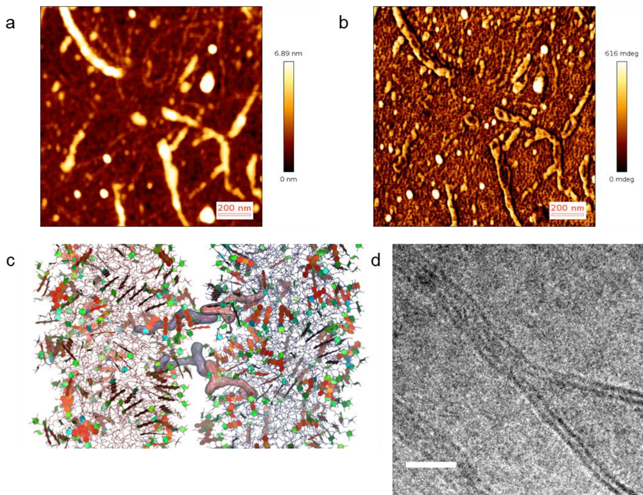
Figure 4. Mechanism of interaction between cylindrical nanoparticles with monovalent anions. (a), (b) AFM pictures obtained in liquid medium of SQ-Dox nanoparticles (2 mM with 2 mM NaCl, scale bar, 200 nm). (a) Height image. (b) Phase image. (c) MD simulations showing inter-cylinders stacking interactions. Stacking pairs from different cylinders are highlighted by semi-transparent surfaces. The colors are the same than in Figure 1. (d) Cryo-TEM pictures showing the stacking of SQ-Dox nanoparticles (2 mM with 2 mM NaCl) to form multilayer structures (Scale bar, 20 nm).
