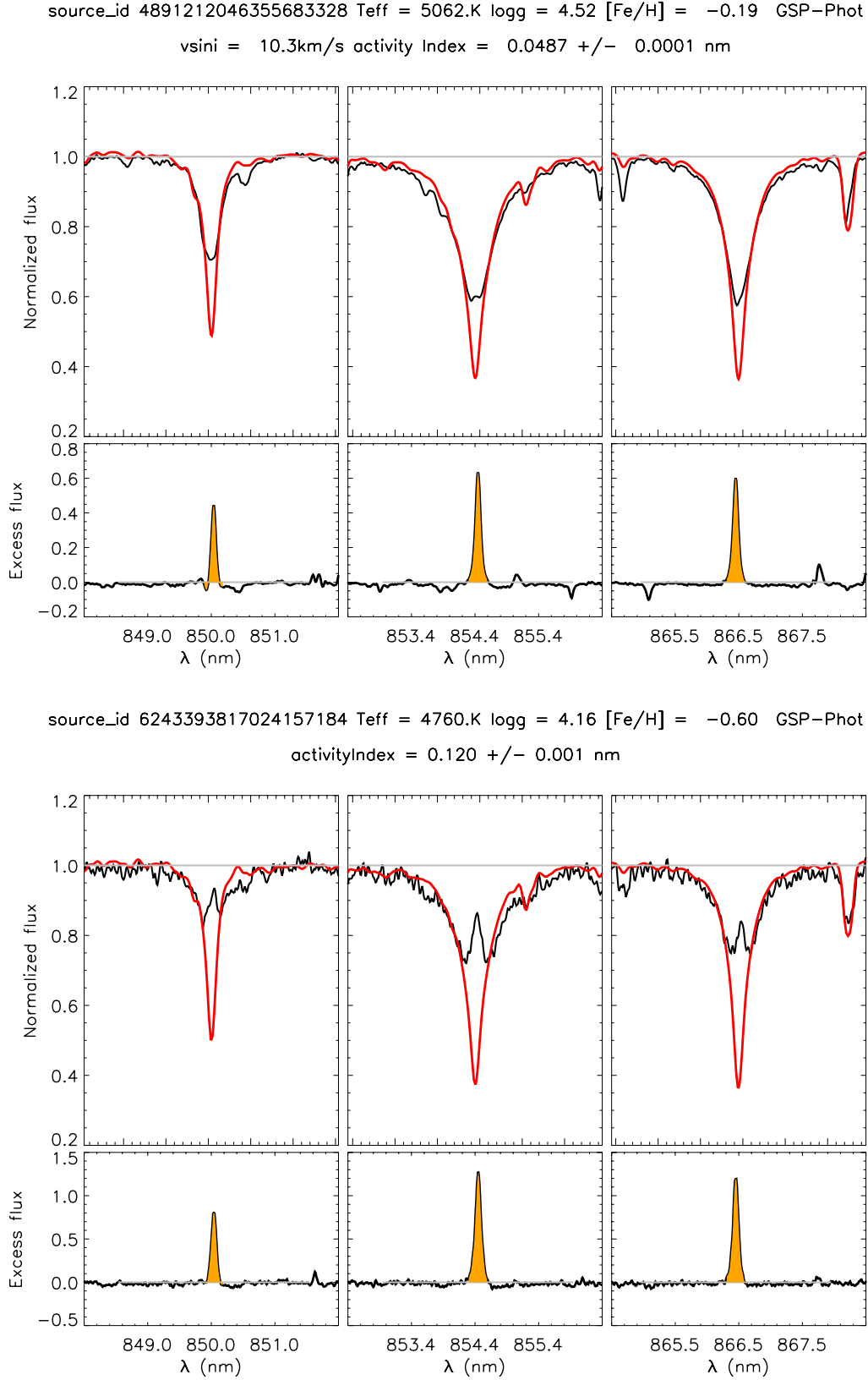
Fig. 22. Examples of the activity index derived by the ESP-CS module. Top panel: Ca II IRT RVS spectrum of the chromospherically active star Gaia DR3 4891212046355683328 (HIP 20737) with a measured R'_{\text{HK}} = -3.72 from FEROS spectra using the Ca H&K doublet. Bottom panel: RVS spectrum for the T Tauri star Gaia DR3 6243393817024157184 with a mass accretion rate of \log \dot{M} = -10.51 M_{\odot} \text{yr}^{-1} . The same method is applied to measure these activity indices for both types of excess flux. Black lines are the observed spectra. Red lines are the purely photospheric spectrum template. The orange filled spectral regions are the area over which the integral of the excess flux is evaluated to produce the activity index.
