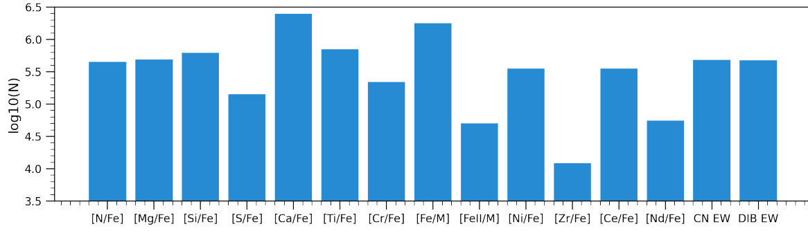
Fig. 17. Histogram showing the number of sources for each chemical species with abundances or equivalent widths in Gaia DR3 produced by the GSP-Spec Matisse-Gaugin method, in logarithmic scale. [\alpha/\text{Fe}] is derived at the same time as the atmospheric parameters ( T_{\text{eff}} , \log g , [\text{M}/\text{H}] ) and is available for approximately 5 million sources. A quality flag flags_gspspec is provided for the best use of the elemental abundances.
