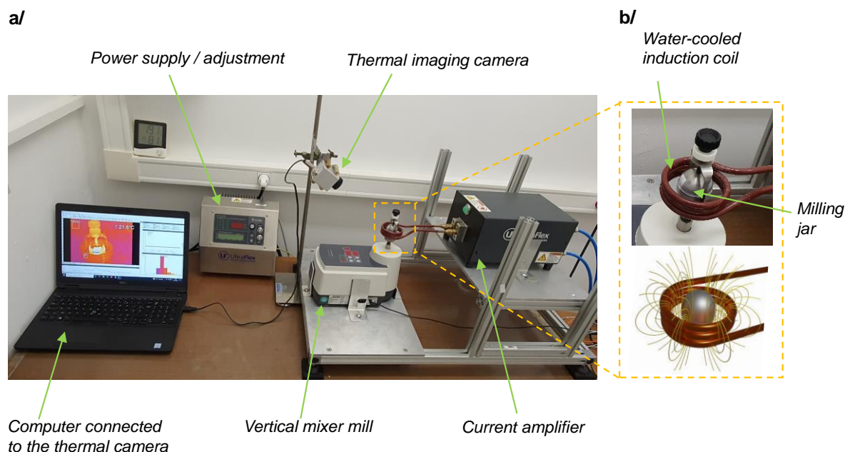
Figure 1. a/ Representation of the experimental set-up used for induction heating during ball-milling (i-BM). b/ Zoom onto the milling jar and induction coil (top), and schematic representation of the magnetic field lines when current is circulating in the coil (bottom). Additional pictures and views of the instrumental set-up are provided in Supporting information (Figure S1).
