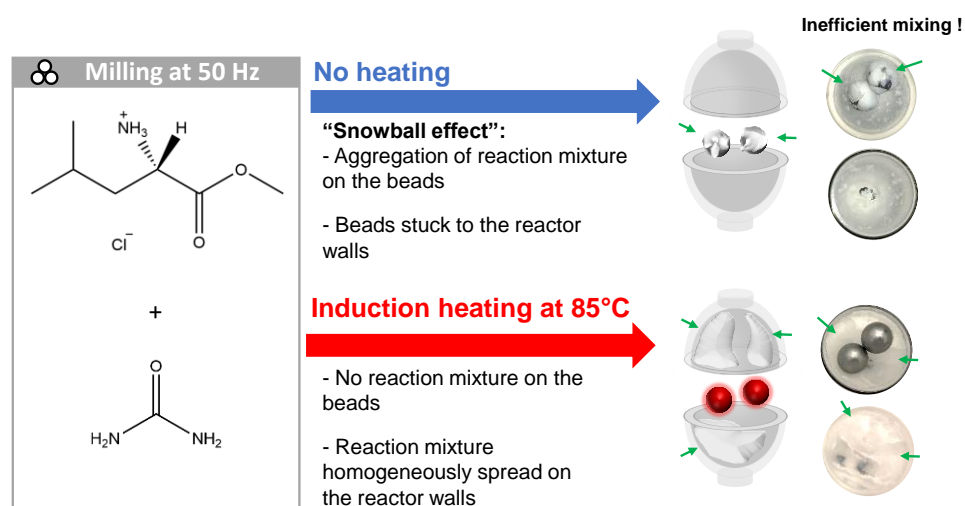
Figure 6. Comparative scheme of the cogrinding of urea (melting point = 133-135°C) with L-leucine methyl ester hydrochloride (melting point = 151-153°C), leading to the formation of a new cocrystal (melting point = 87-92°C). On top, in absence of i-BM, the snowball phenomenon occurs after 4-5 min of milling at 50Hz. On the bottom, when using i-BM to quickly heat the two ss beads through the PMMA jar up to 85°C in a few seconds, the formation of the snowball is prevented. A video showing the formation of the “snowball”, and its subsequent disappearance under i-BM is provided in SI.
