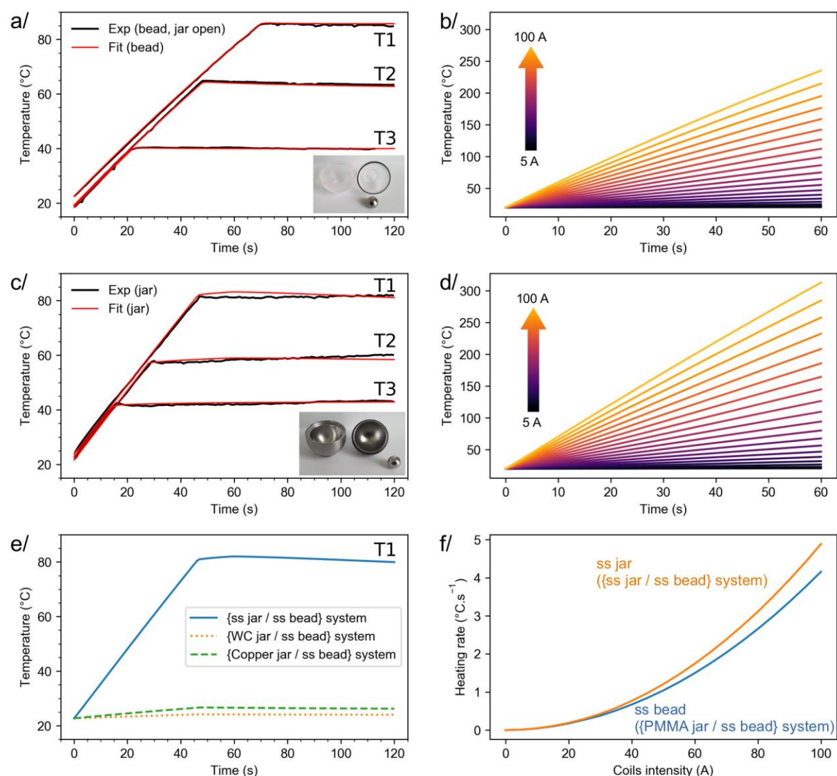
Figure 3. On the left, experiments and fits performed on the {PMMA jar / ss bead} (a) and {ss jar / ss bead} (c) systems used for induction heating during ball-milling, showing that the temperature of the jar or bead can be stabilized at different values (noted here T1, T2 and T3), depending on the i-BM parameters. On the right, simulations performed on the {PMMA jar / ss bead} (b) and {ss jar / ss bead} (d) systems, showing the influence of the coils' current on the maximum temperature achieved, and on the heating rate. e/ Simulations with the same condition as the {ss jar / ss bead} system stabilized at the T1 temperature, when other jar materials are used. f/ Initial heating rate (at t = 0 s) as a function of the intensity in the coils, for the {ss jar / ss bead} and {PMMA jar / ss bead} systems. All parameters used in simulations are given in supporting information in Tables S1 (current as a function of the time) and S2 (parameters related to the materials' properties).
