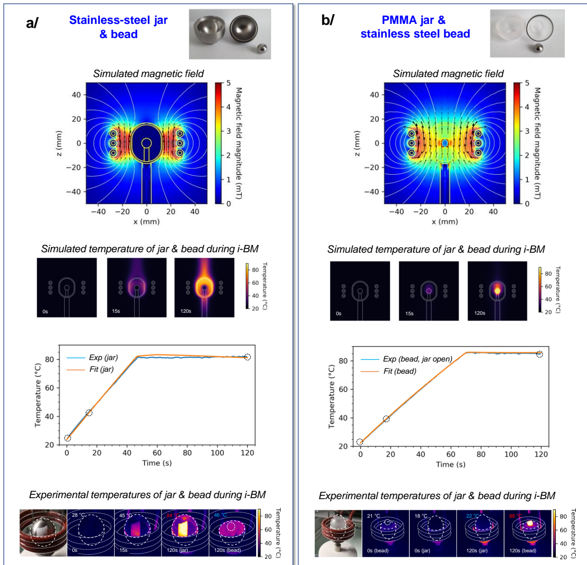
Figure 2. Simulations and experiments performed on the two systems used for induction heating during ball-milling (i-BM) : a/ {ss jar / ss bead} and b/ {PMMA jar / ss bead}. The experimental and simulation parameters used are provided in supporting information (Tables S1 et S2). Top : simulated magnetic field lines ; Middle : simulations of the changes in temperature during i-BM at different time points, and graphical comparison of experimental and fitted temperatures of jar (left) and bead (right) during i-BM. Bottom : photos and thermal images during i-BM, at the time-points indicated by circles on the graphs above, showing that after 120 s of i-BM, the temperature of the beads is moderate in a/ ( i.e. lower than the temperature of the jar), but high in b/ ( i.e. much higher than that of the jar). To enable temperature measurements on stainless steel using the IR-thermal imaging camera, a sticker was added on the jar (or bead), as discussed in supporting information (Figures S2 & S6).
