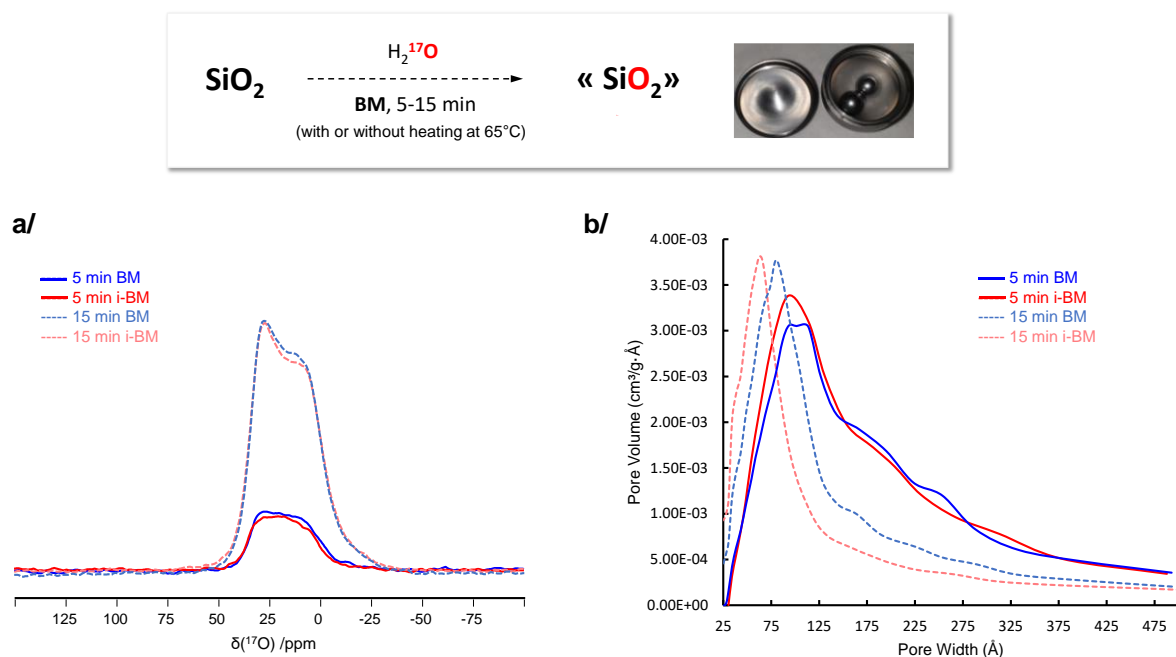
Figure 4. Influence of i-BM on the isotopic labeling of fumed silica. a/ ^{17}\text{O} MAS NMR spectra, and b/ comparison of the pore size distribution (as determined from \text{N}_2 adsorption measurements), for phases prepared after 5 and 15 minutes milling, with (red) or without (blue) i-BM.
