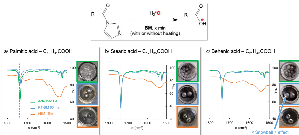
Figure 5. Influence of i-BM on the isotopic labeling of fatty acids, as demonstrated using IR spectroscopy, for a/ palmitic acid ( T_{\text{melt}} \approx 73^\circ\text{C} ; T_{\text{i-BM}} = 70^\circ\text{C} ), b/ stearic acid ( T_{\text{melt}} \approx 78^\circ\text{C} ; T_{\text{i-BM}} = 85^\circ\text{C} ), and c/ behenic acid ( T_{\text{melt}} \approx 90^\circ\text{C} ; T_{\text{i-BM}} = 90^\circ\text{C} ). IR spectra of the activated FA (green), BM-hydrolysis test at room-temperature (blue, after 60 min milling) and under i-BM conditions (orange, after 15 min milling) are shown, with the dashed vertical line pointing to the C=O stretching frequency of the activated FA. Hydrolysis reactions were optimized using non-labeled or ^{18}\text{O} -enriched water (to check the feasibility of i-BM reactions), prior to working with ^{17}\text{O} -enriched water, in line with our previous work (which had shown that no isotopic effect on the hydrolysis rate would occur upon switching to ^{17}\text{O}/^{18}\text{O} -enriched water). Characterizations by mass-spectrometry of oxygen-labeled compounds are provided in supporting information, together with ^1\text{H} solution NMR analyses confirming the purity of the isolated products (Figures S9 to S13 in ESI).
