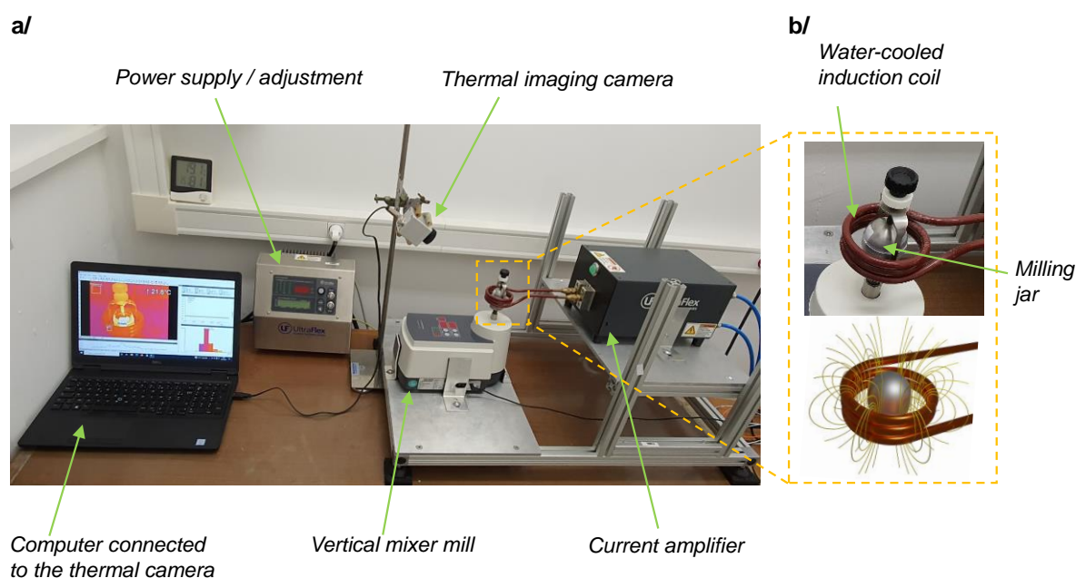
Figure 1. a/ Representation of the experimental set-up used for induction heating during ball milling (i-BM). b/ Zoom onto the milling jar and induction coil (top), and schematic representation of the magnetic field lines when current is circulating in the coil (bottom). Additional pictures and views of the instrumental set-up are provided in Supporting information (Figure S1).
