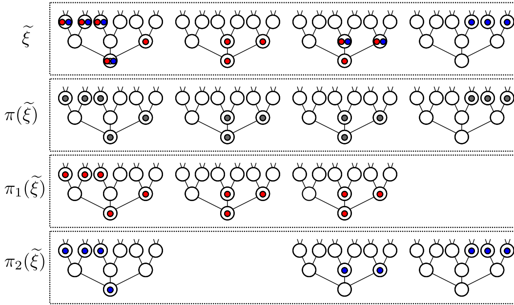
Figure 1: A two-type herds configuration \tilde{\xi} is depicted on top, with the two types represented in blue and red (it is assumed that in the four herds of this configuration, no particle is present other than the ones depicted). The projections \pi(\tilde{\xi}) , \pi_1(\tilde{\xi}) and \pi_2(\tilde{\xi}) are shown in the second, third and fourth rows, respectively.
