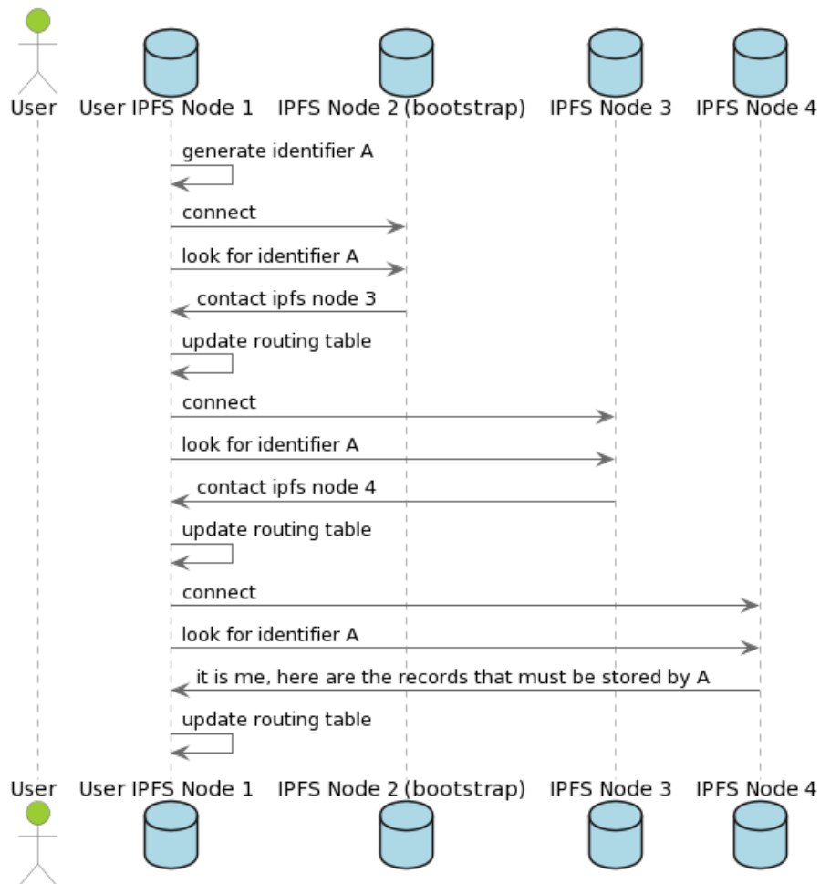
Fig. 1: Sequence diagram for the connection of a new node.
